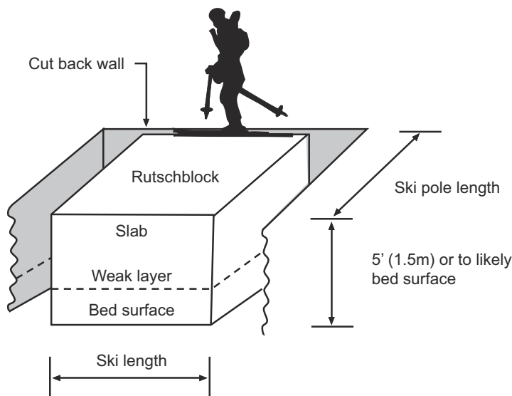
Figure 1-5. Rutschblock Test.
