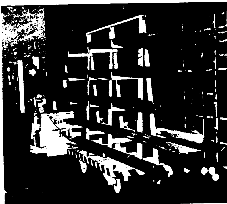
Figure 5-53. Tree frame racks mounted on warehouse trailer.
