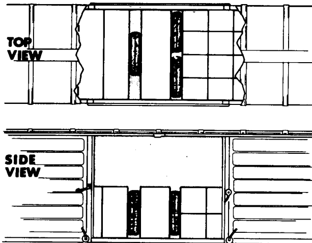
Figure 3-47. Multiple void bracing with pneumatic dunnage units.
