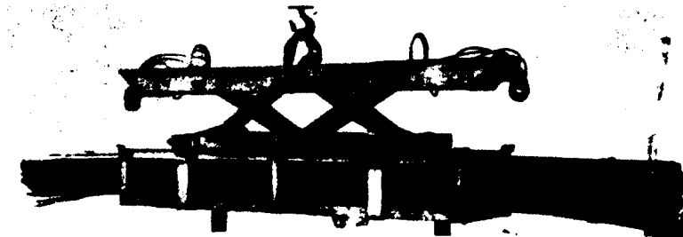
Figure 5-55. Automatic grab hook and spreader beam.
