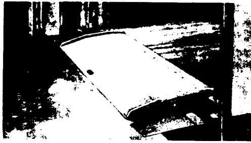
Figure 4-68. Dockboard in operating position.
