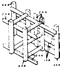
Figure 3-35. Front bulkhead—positioned in trailer, detail of bulkhead.
