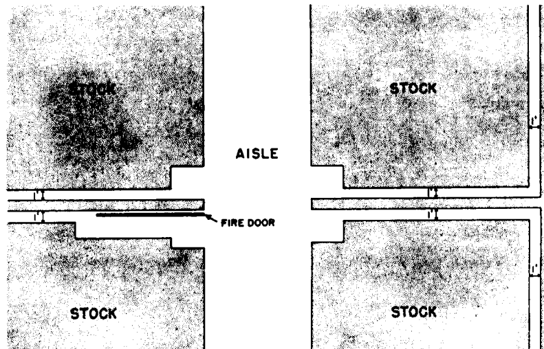
Figure 6-5. Stock clearance at walls for material subject to excessive swelling.
