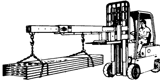
Figure 4-54. Crane boom attached to forklift truck.
