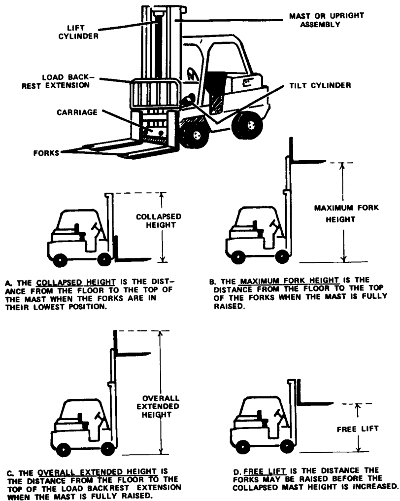
Figure 4-112. The mast or upright is the elevating assembly of a fork lift truck.
