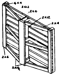
Figure 3-32. Examples of right and wrong truck loading.
