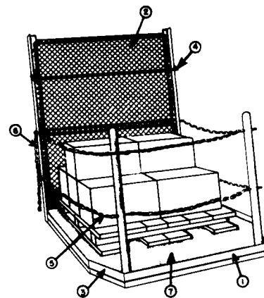
Figure 4-59. Features of the safety pallet.
