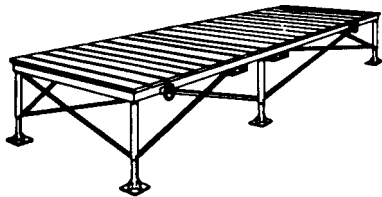
Figure 4-71. Portable platform.
