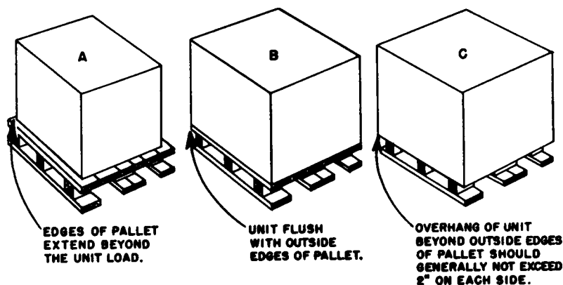
Figure 3-20. Prevention of chafing.
