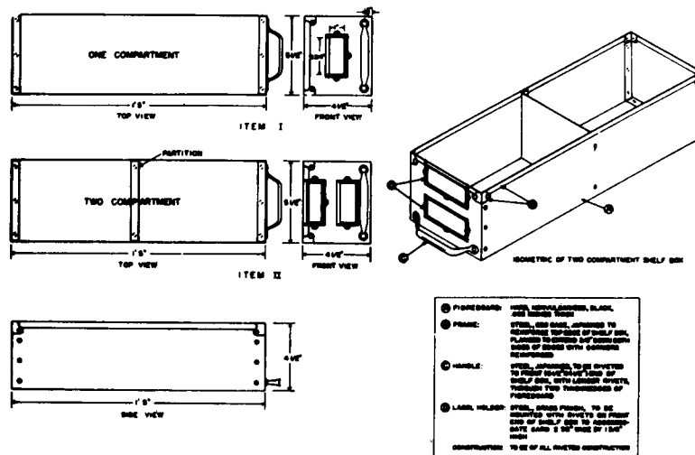
Figure 2-33. Shelf Box, Small, One and Two Compartment
