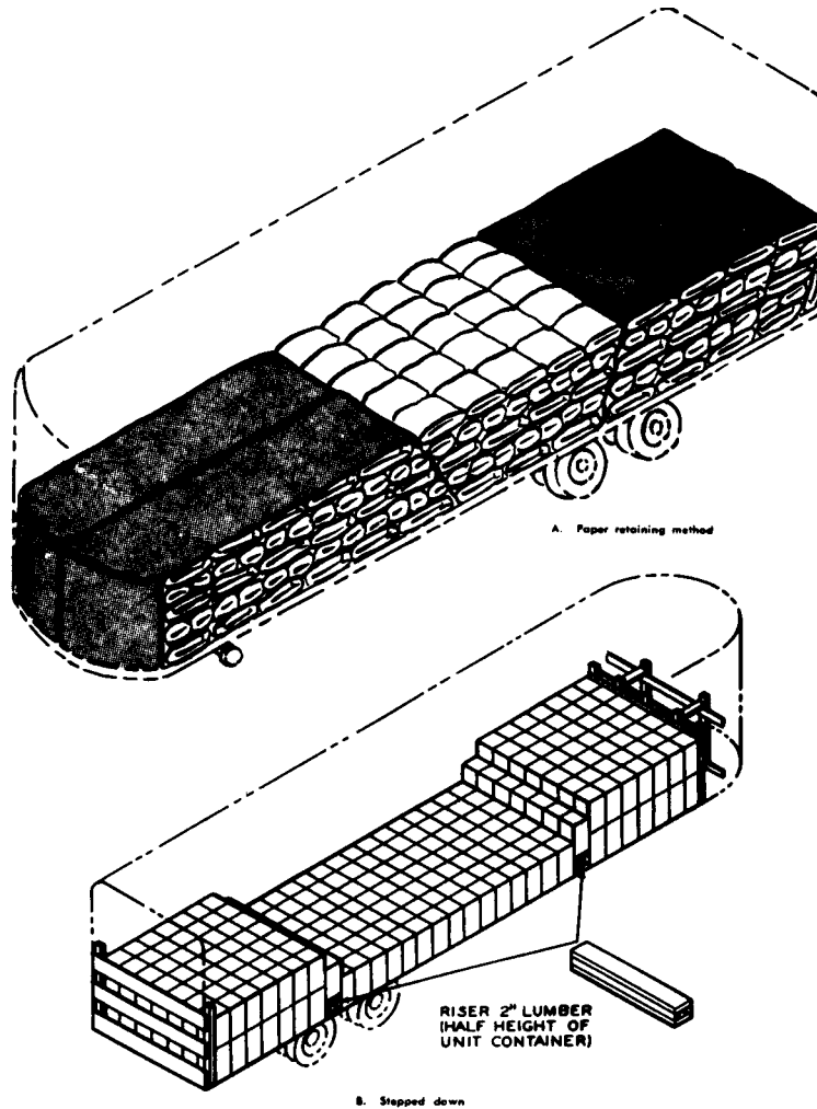
Figure 3-40 Loading
