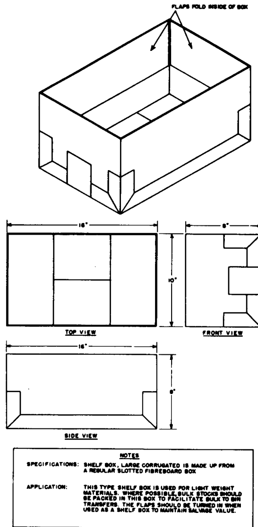
Figure 2-35. Large Corrugated Shelf Box
