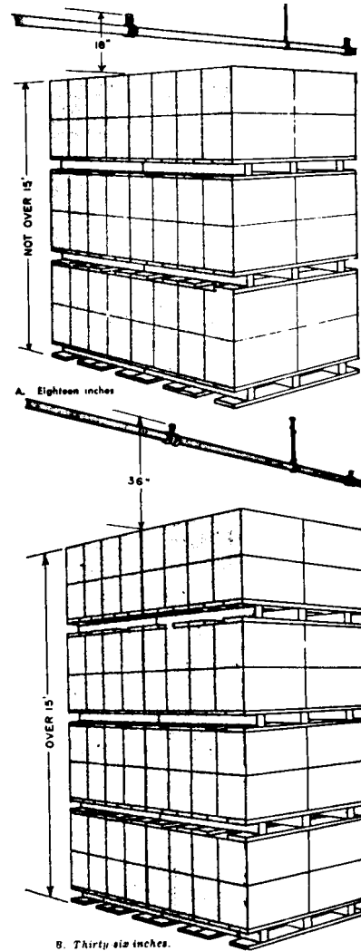
Figure 6-1. Overhead stack clearance at sprinkler head.
