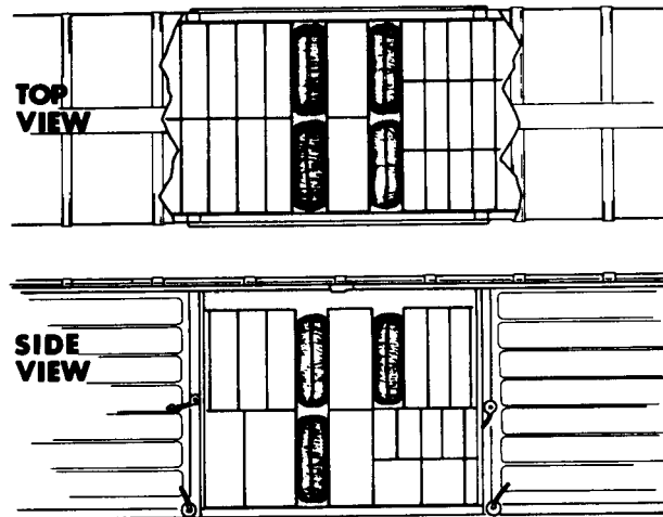
Figure 3-48. Pneumatic dunnage units in various void arrangements.
