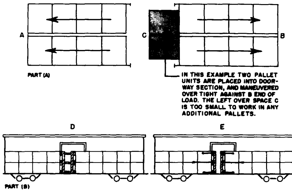
Figure 3-22. Palletized loads.
