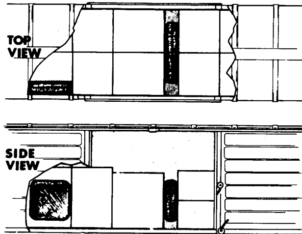
Figure 3-50. Pneumatic dunnage stays load laterally and longitudinally.
