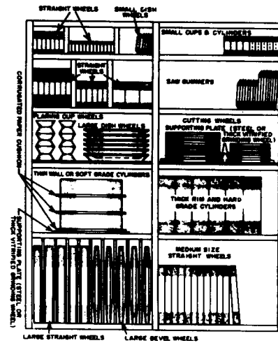
Figure 5-46. Bin storage of grinding wheels.
