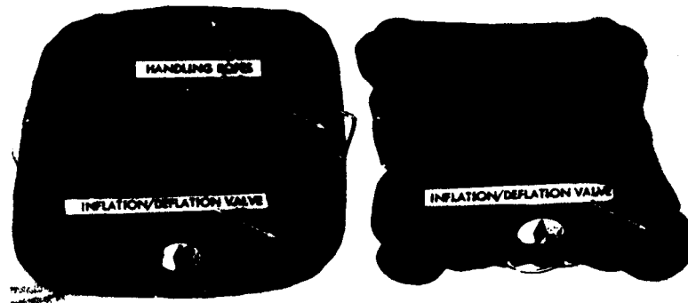
Figure 3-42. Reusable pneumatic dunnage unit complete.
