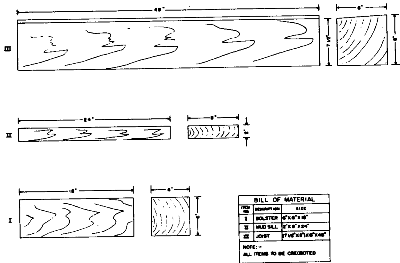
Figure 5-12. Diagram of lumber foundation components.
