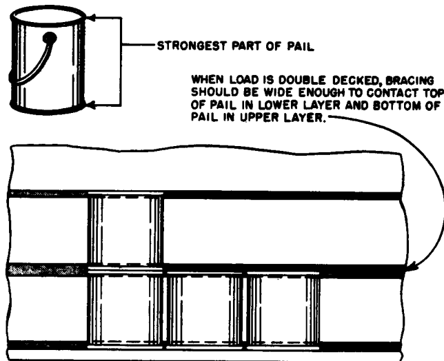
Figure 3-25. Placing of last two pallets.
