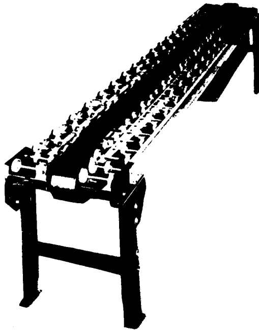
Figure 4-39. Conveyor, accumulation, dual-actuator.
