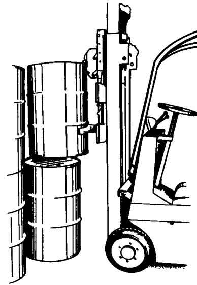
Figure 4-48. Drum-handling attachment single-drum type, vertical carry.
