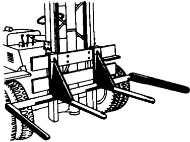
Figure 4-47. Drum-handling attachment.
