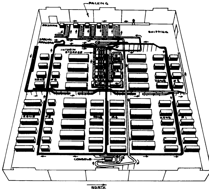
Figure 2-42. Layout Containing an Automated Materials Handling System
