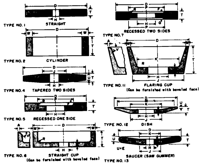
Figure 5-47. Typical types of grinding wheels.
