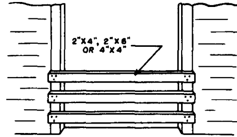
Figure 3-13. Doorway protection for rough freight only.
