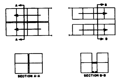
Figure 3-21. Floor supports.
