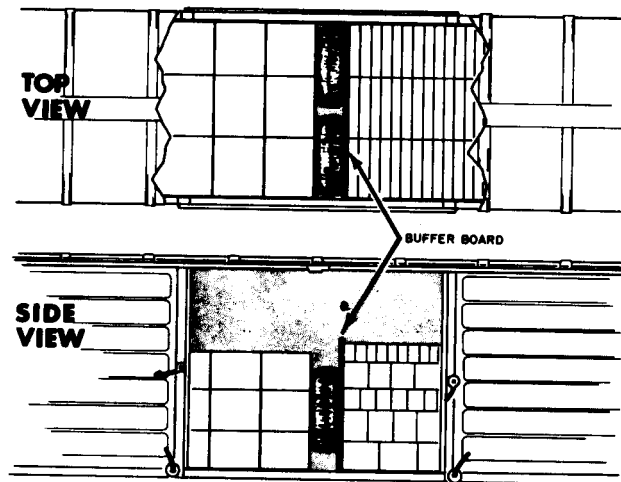
Figure 3-51. Buffer board insertions.
