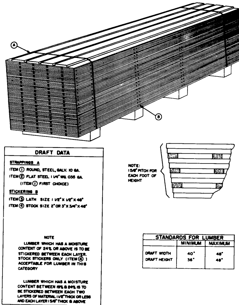
Figure 5-3. Diagram outlining draft requirements for outdoor storage.
