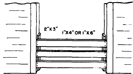
Figure 3-14. Flush doorway protection for cars with wooden doorposts.
