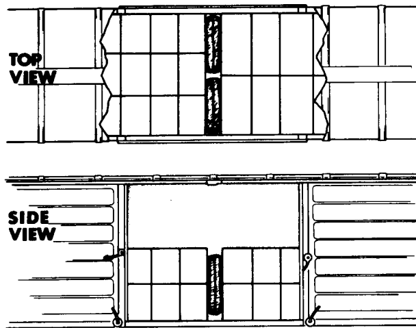
Figure 3-45. Single void pneumatic dunnage bracing pattern.
