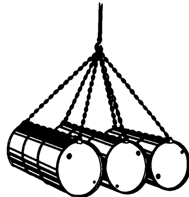
Figure 4-46. Drum-handling sling.
