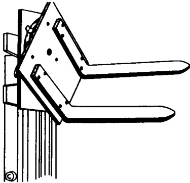
Figure 4-56. Revolving carriage.
