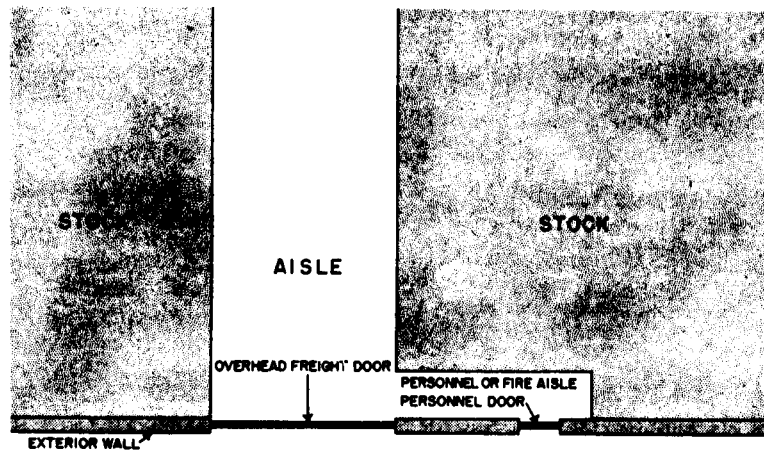
Figure 6-4. Stock clearance at exterior walls (nonhazardous materials).
