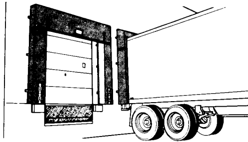
Figure 4-70. Dock seal head pad.
