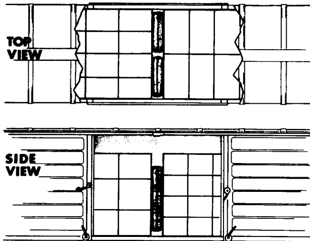
Figure 3-46. Larger dunnage units bracing higher loads.
