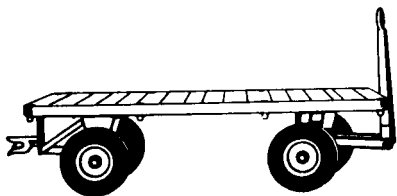
Figure 4-32. Trailer, platform, warehouse, 6,000-pound, pneumatic tires.
