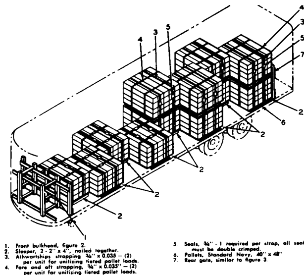
Figure 3-41. Staggered palletized loading.
