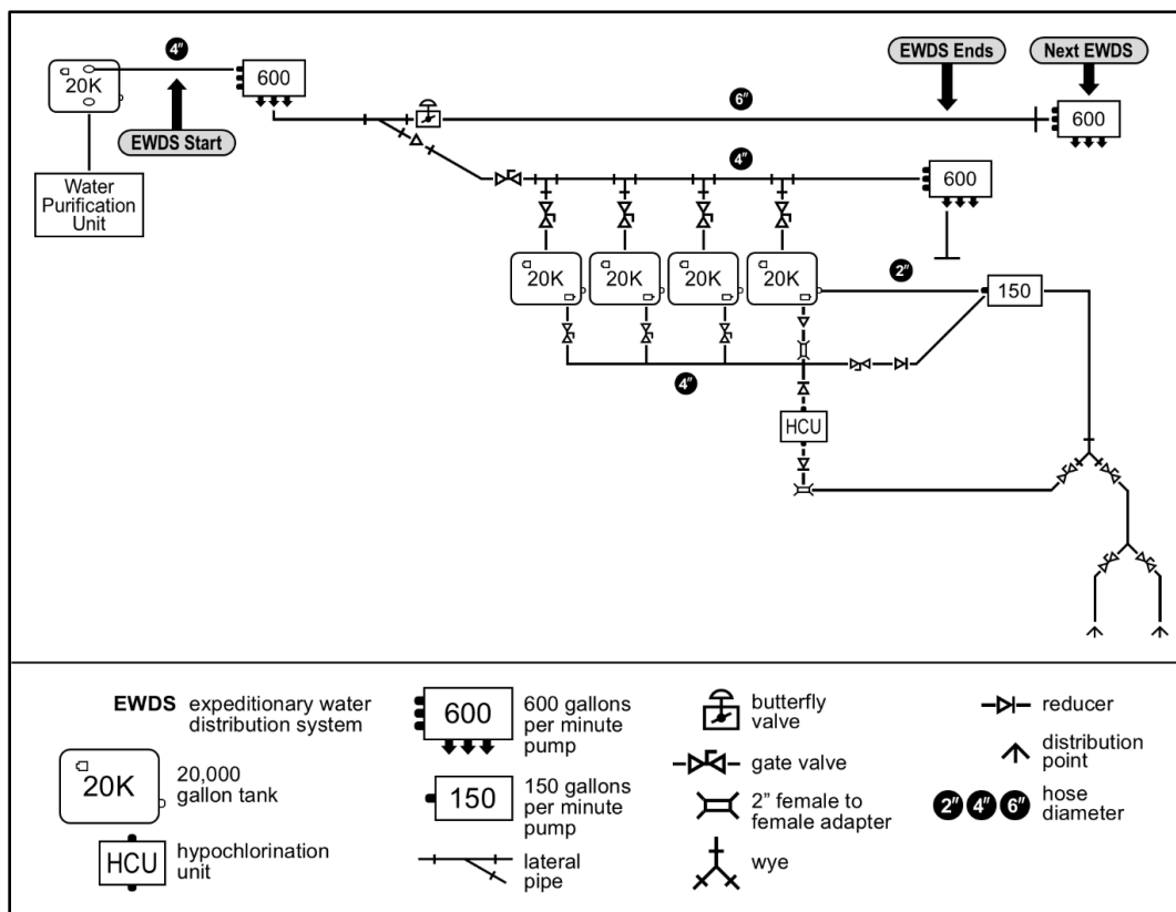
Figure A-11. Design for operational use of the EWDS
