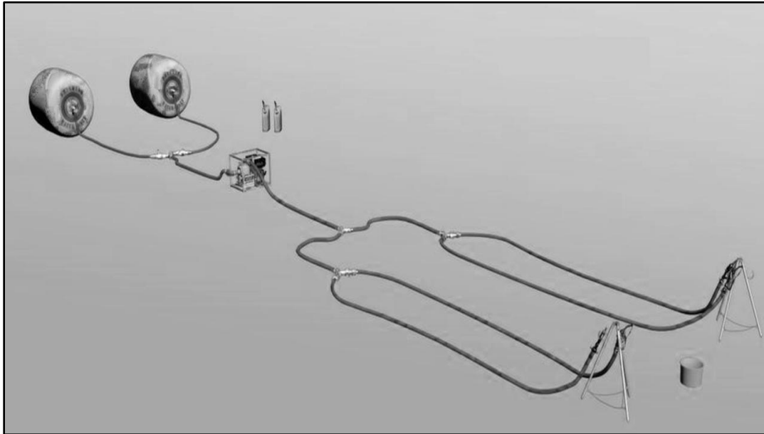
Figure A-12. Forward area water point supply system
