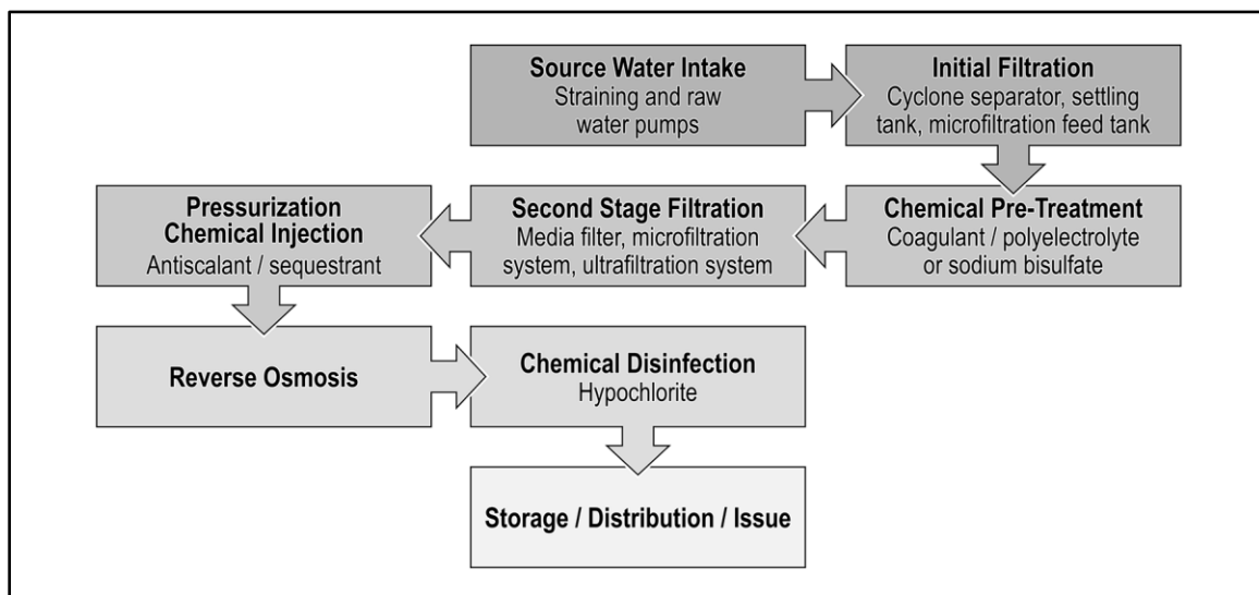
Figure E-1. Water treatment process
