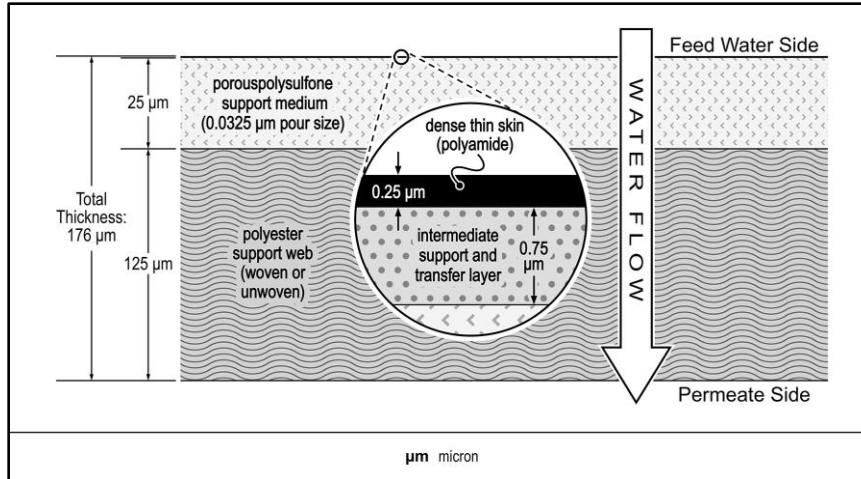
Figure E-3. Reverse osmosis membrane composition
