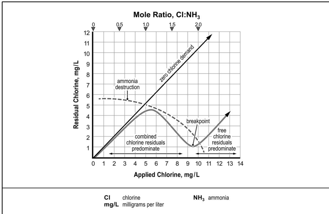
Figure E-5. Breakpoint chlorination chart
