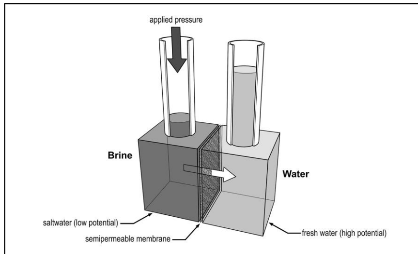
Figure E-2. Reverse osmosis process
