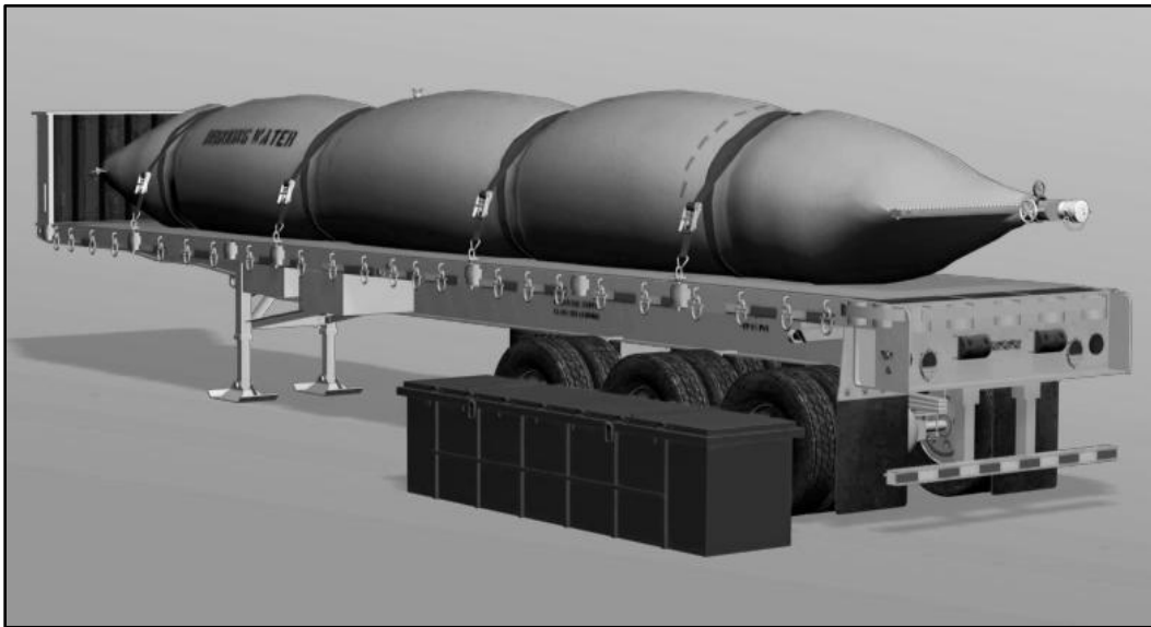
Figure A-14. Semi-trailer mounted fabric tank
