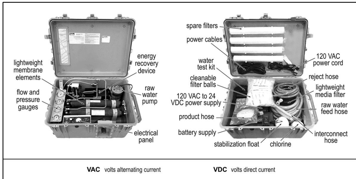
Figure A-6. Platoon water purification system
