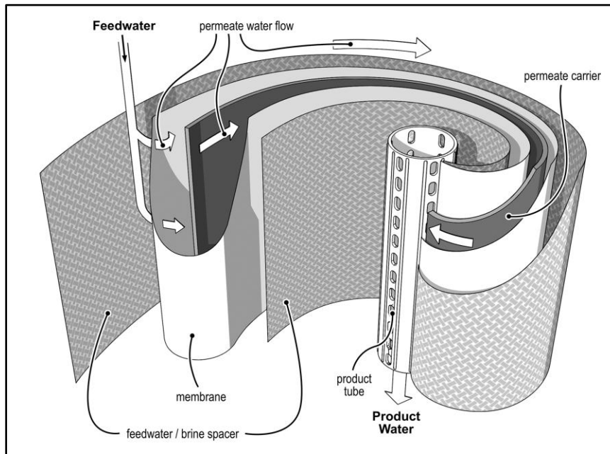
Figure E-4. Spirally wound reverse osmosis membrane assembly
