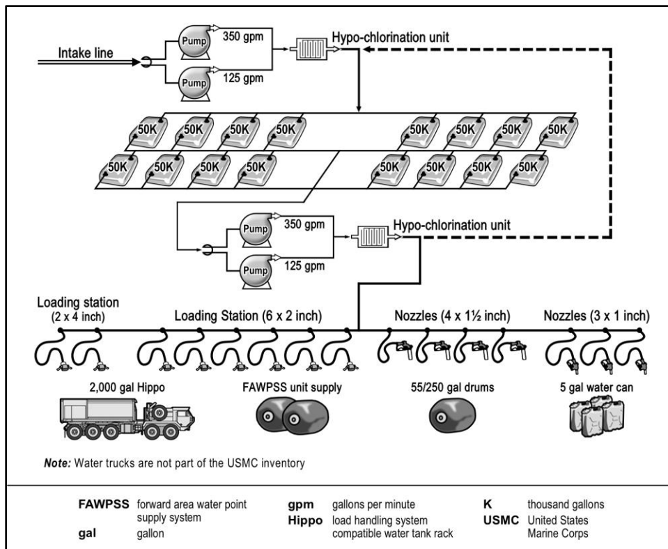
Figure A-8. 800,000-gallon water storage and distribution system
