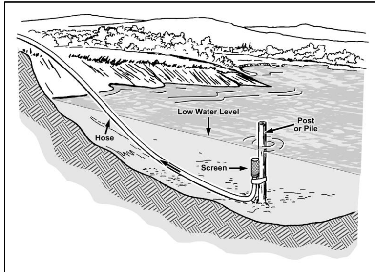
Figure B-3. Stake method
