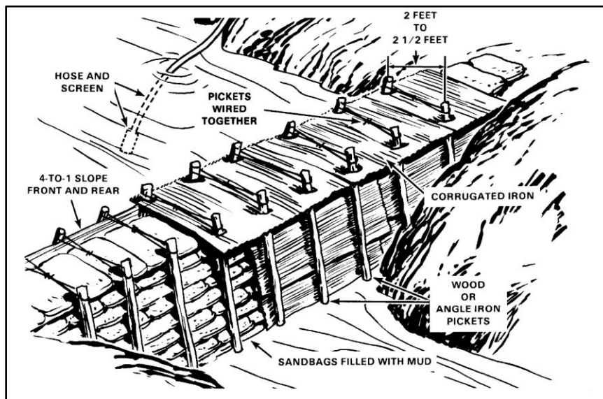
Figure B-6. Improvised dam
