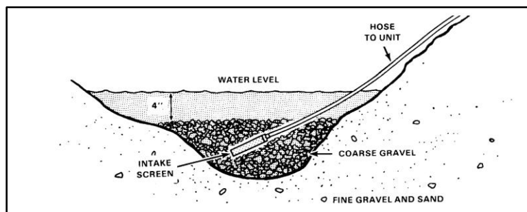
Figure B-4. Gravel pit method
