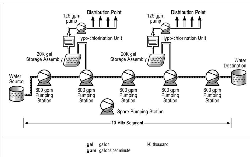
Figure A-9. Tactical water distribution system
