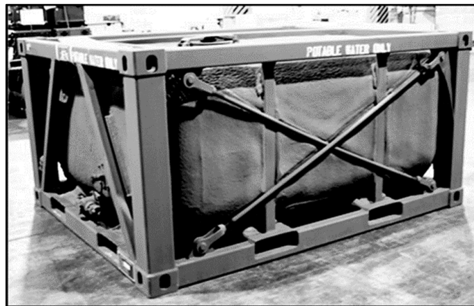
Figure A-16. Marine Corps water six container storage tank module
