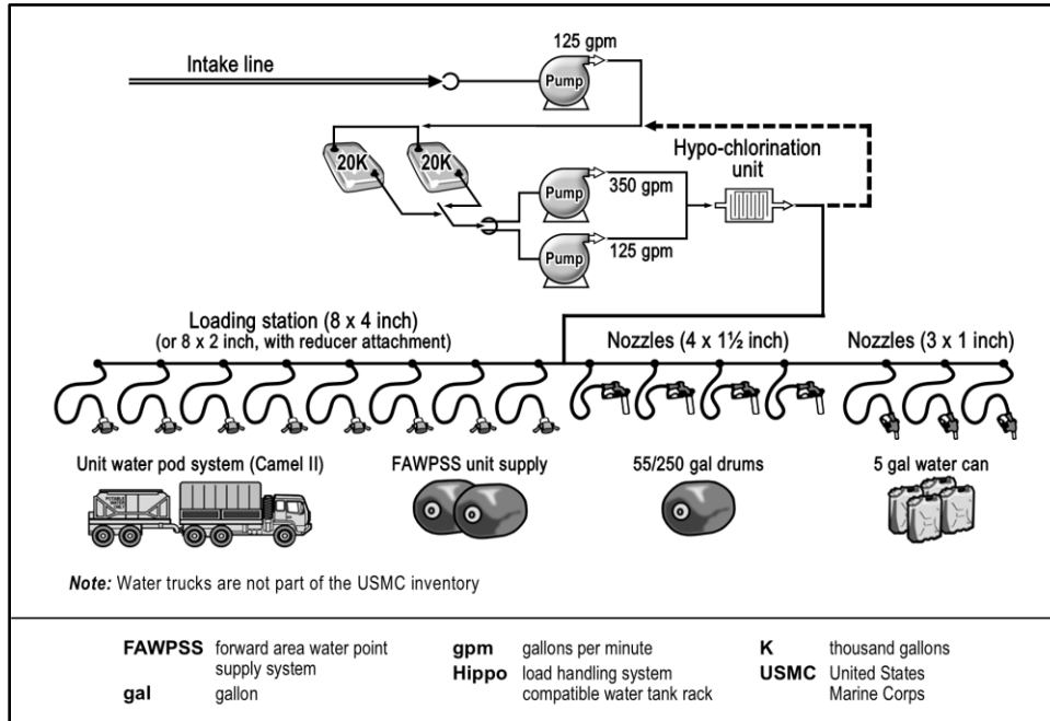
Figure A-7. 40,000-gallon water storage and distribution system
