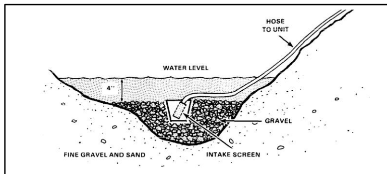
Figure B-5. Gravel pit method with bucket
