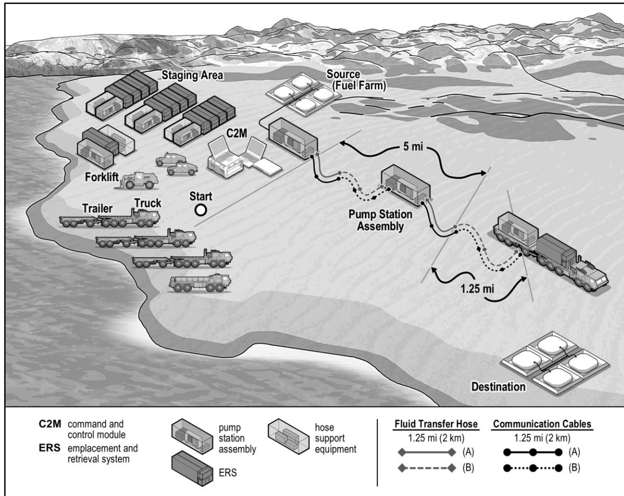
Figure A-18. Early entry fluid distribution system
