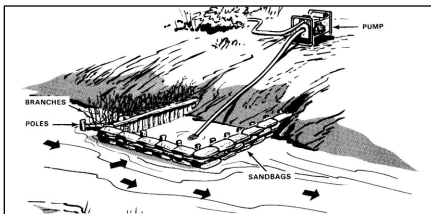
Figure B-7. Baffle dam
