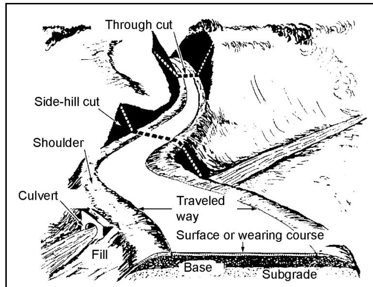
Figure 4-19. Parts of a road
