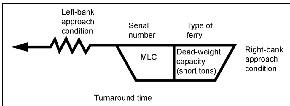
Figure 5-3. Ferry symbols
