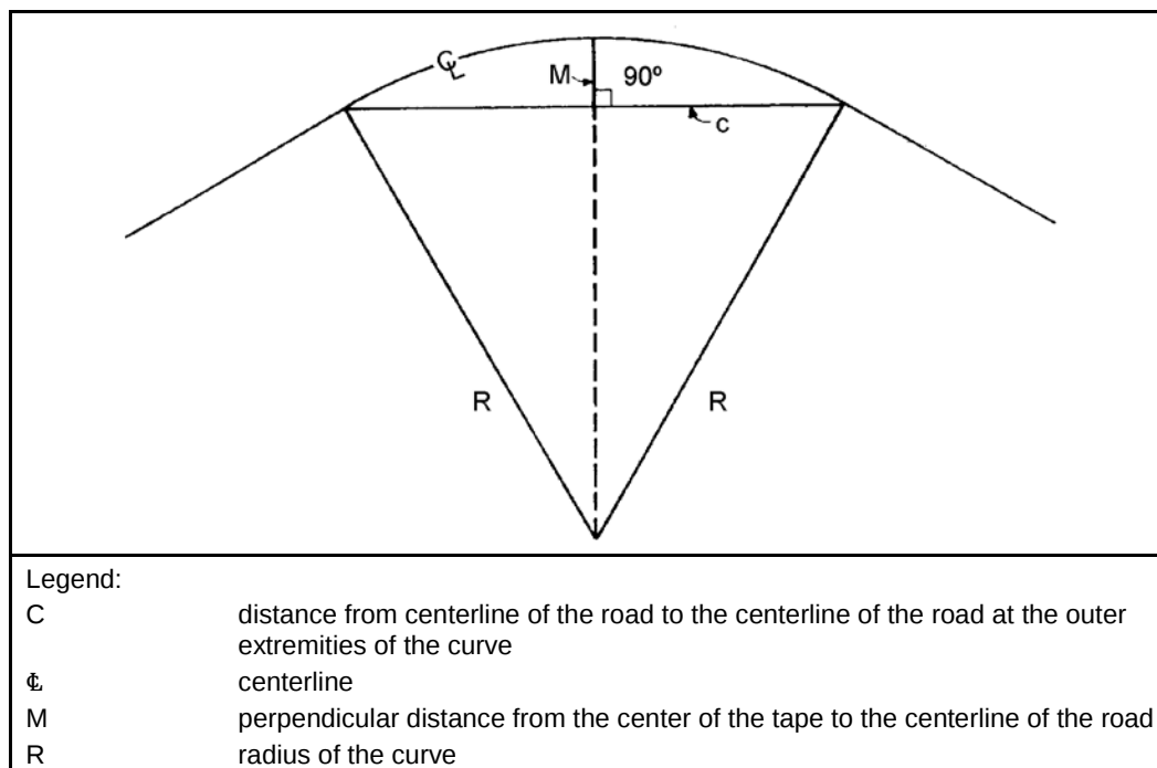
Figure 4-5. Cord method
