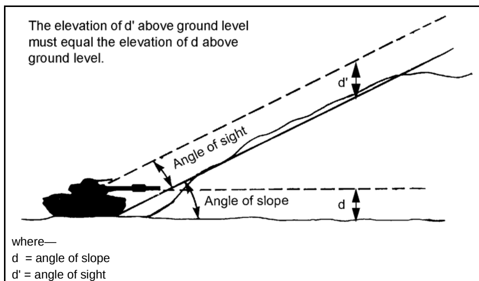
Figure 4-10. Angle-of-slope method to determine percent of slope
