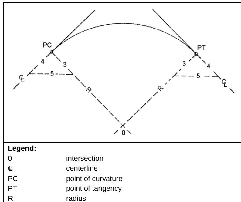
Figure 4-4. Triangulation method
