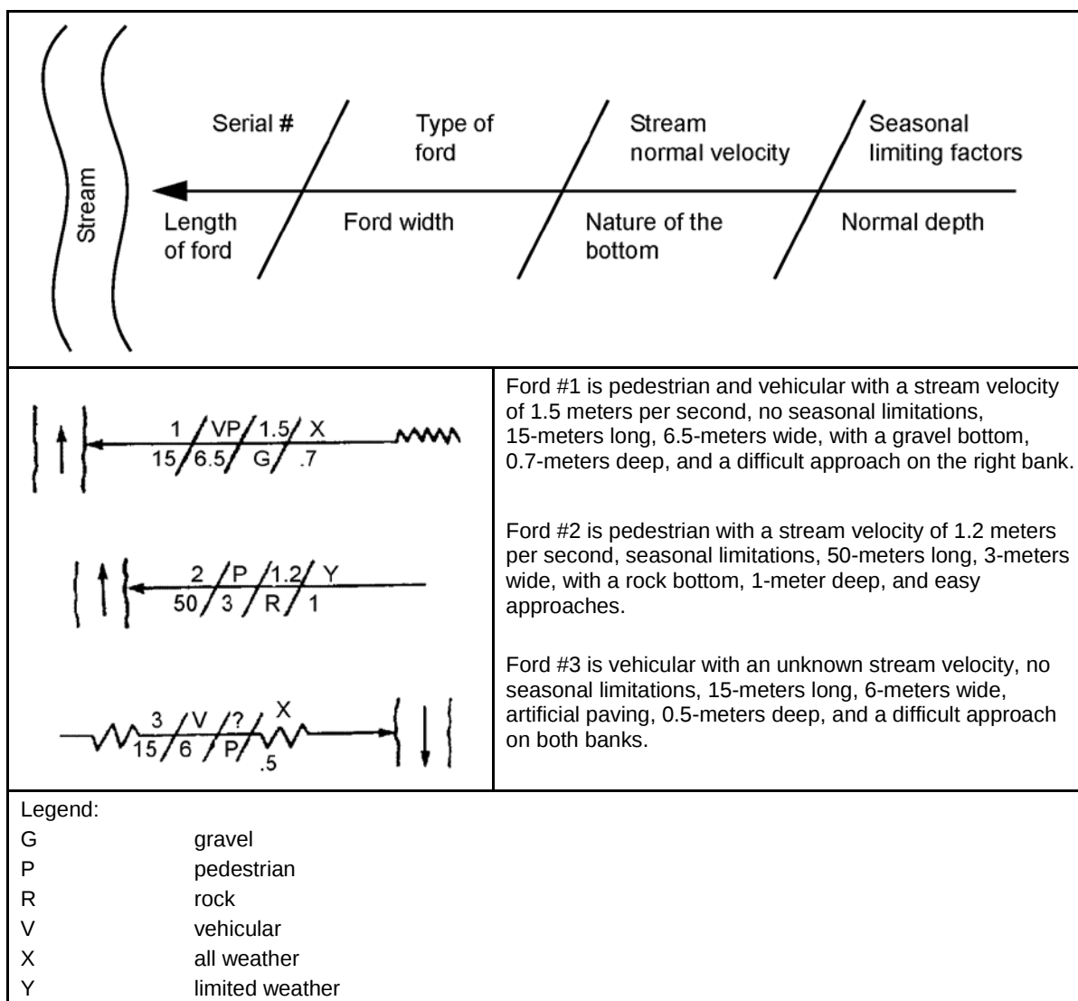
Figure 5-2. Ford symbols
