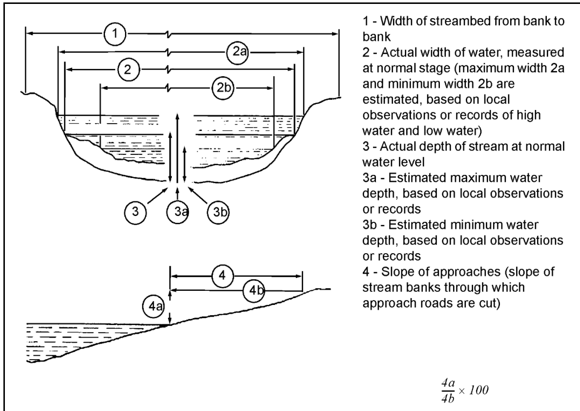
Figure 5-5. Dimensions required for streams and rivers
