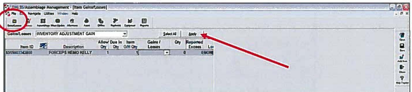
Figure 1.20 Items Gains/Losses
