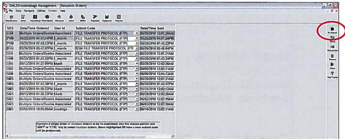
Figure 1.30 Resubmit Orders
