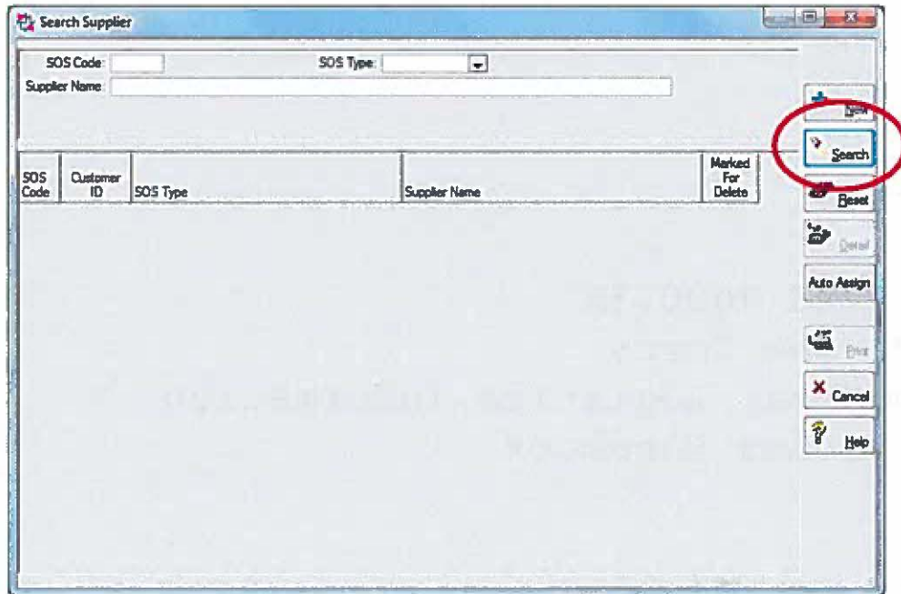
Figure 1.16 Search Supplier
