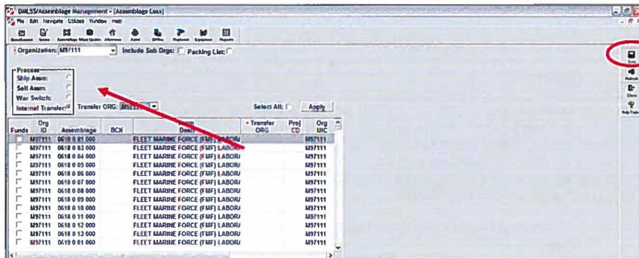
Figure 1.7 Assemblage Loss
