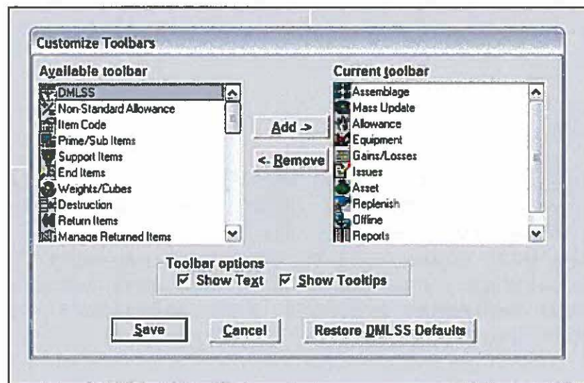
Figure 1.2 Customization Toolbar
