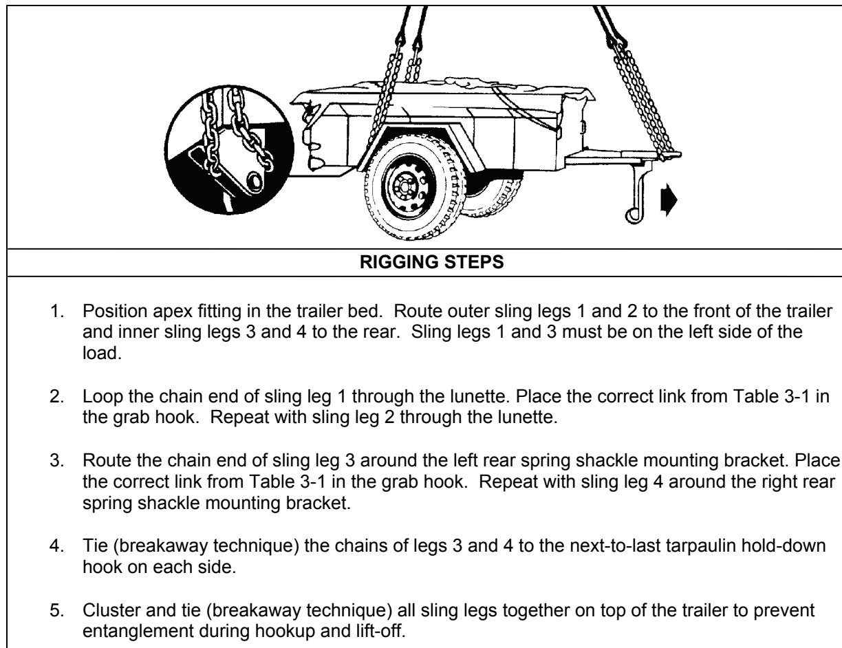
Figure 3-1. M416 1/4-Ton Trailer
