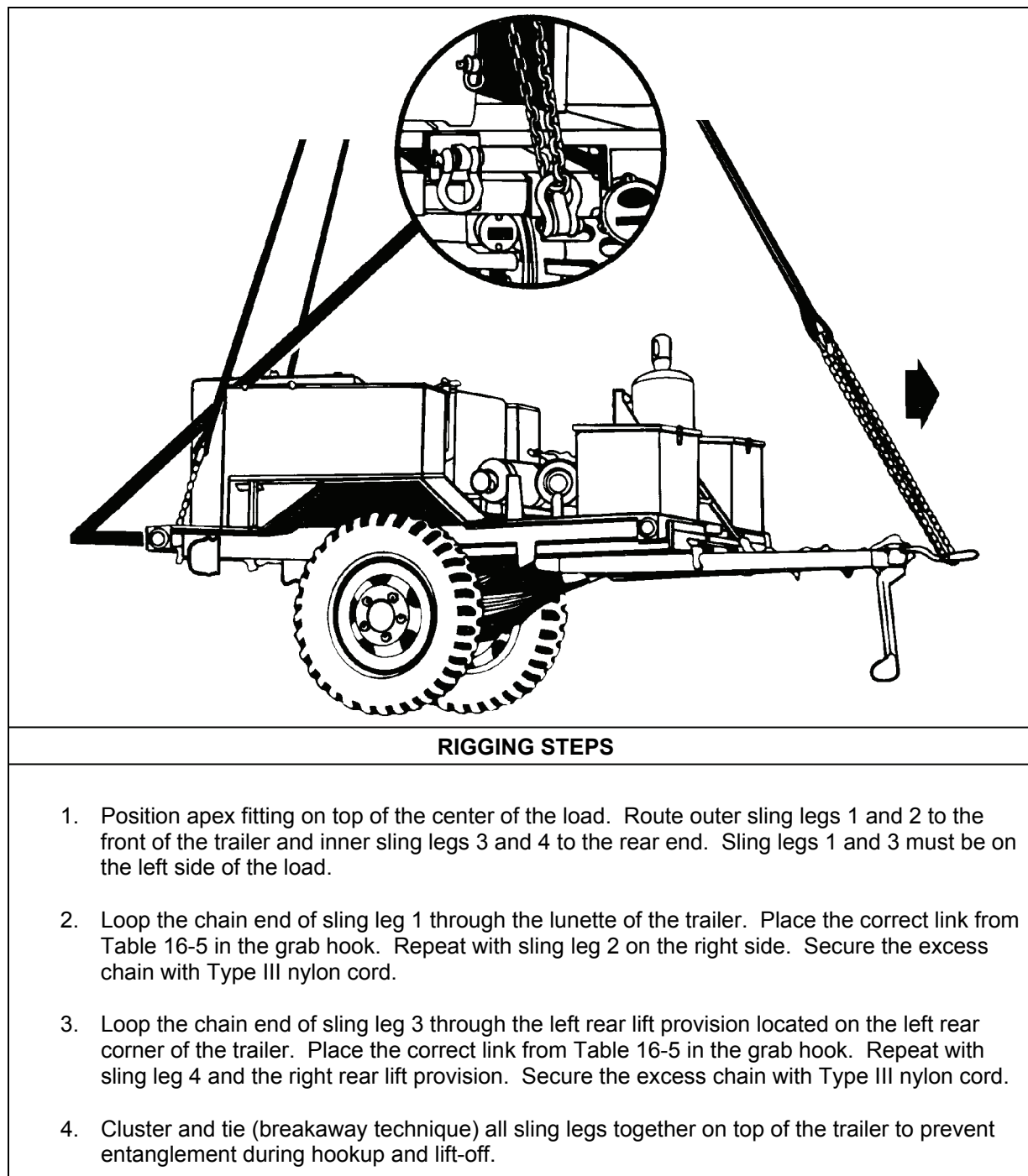
Figure 16-5. Trailer-Mounted Welding Shop
