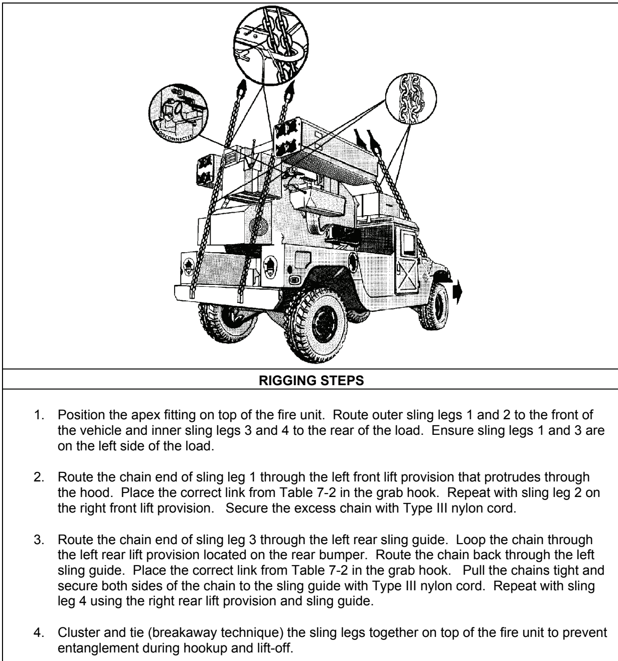
Figure 7-2. Avenger on M1097/M1097A1/M1097A2 HMMWV with ECU/PPU and an Aluminum Airlift Bumper with or without Bustle Box Stowed on the Roof
