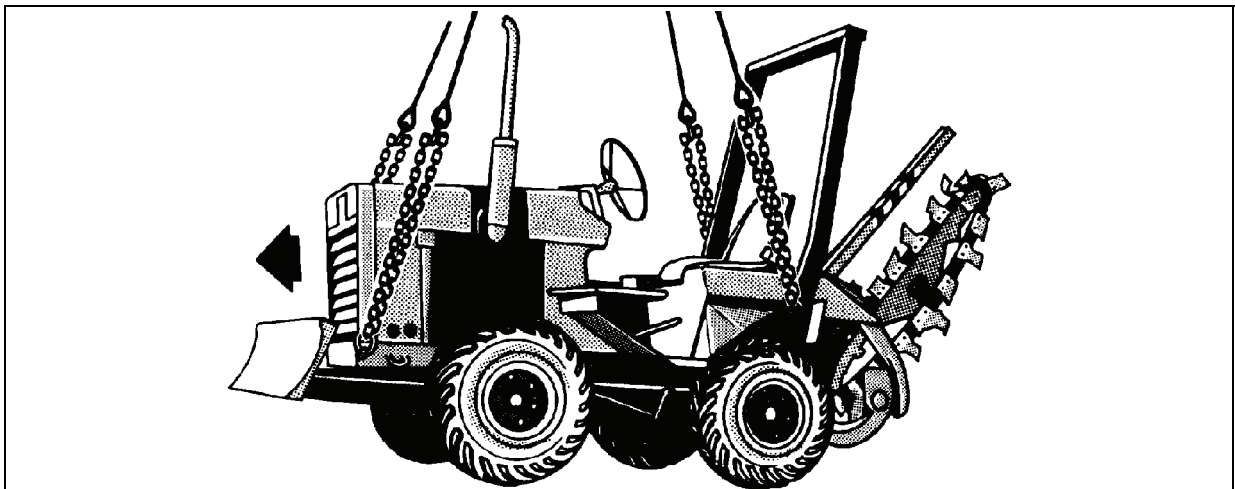
Figure 8-8. Ditching Machine
