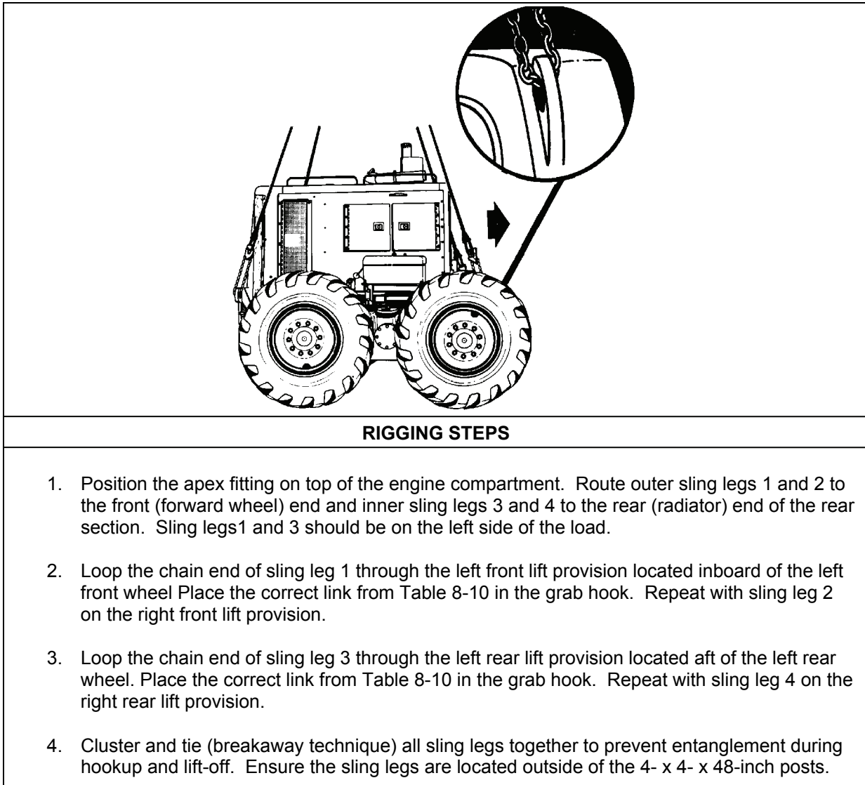
Figure 8-10a. 130GS Grader (Rear Section)
