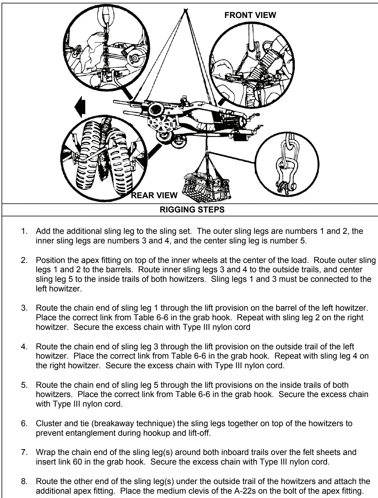
Figure 6-6. Two M102 105-MM Howitzers with One, Two, or Three A-22 Cargo Bags
