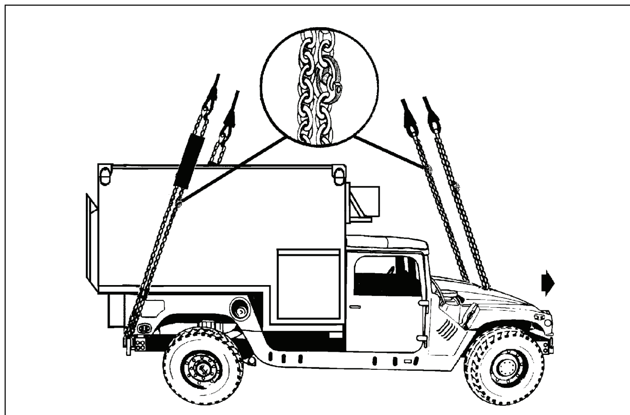
Figure 2-12. M1097/M1113 with Gitchner Model 1497A Shelter
