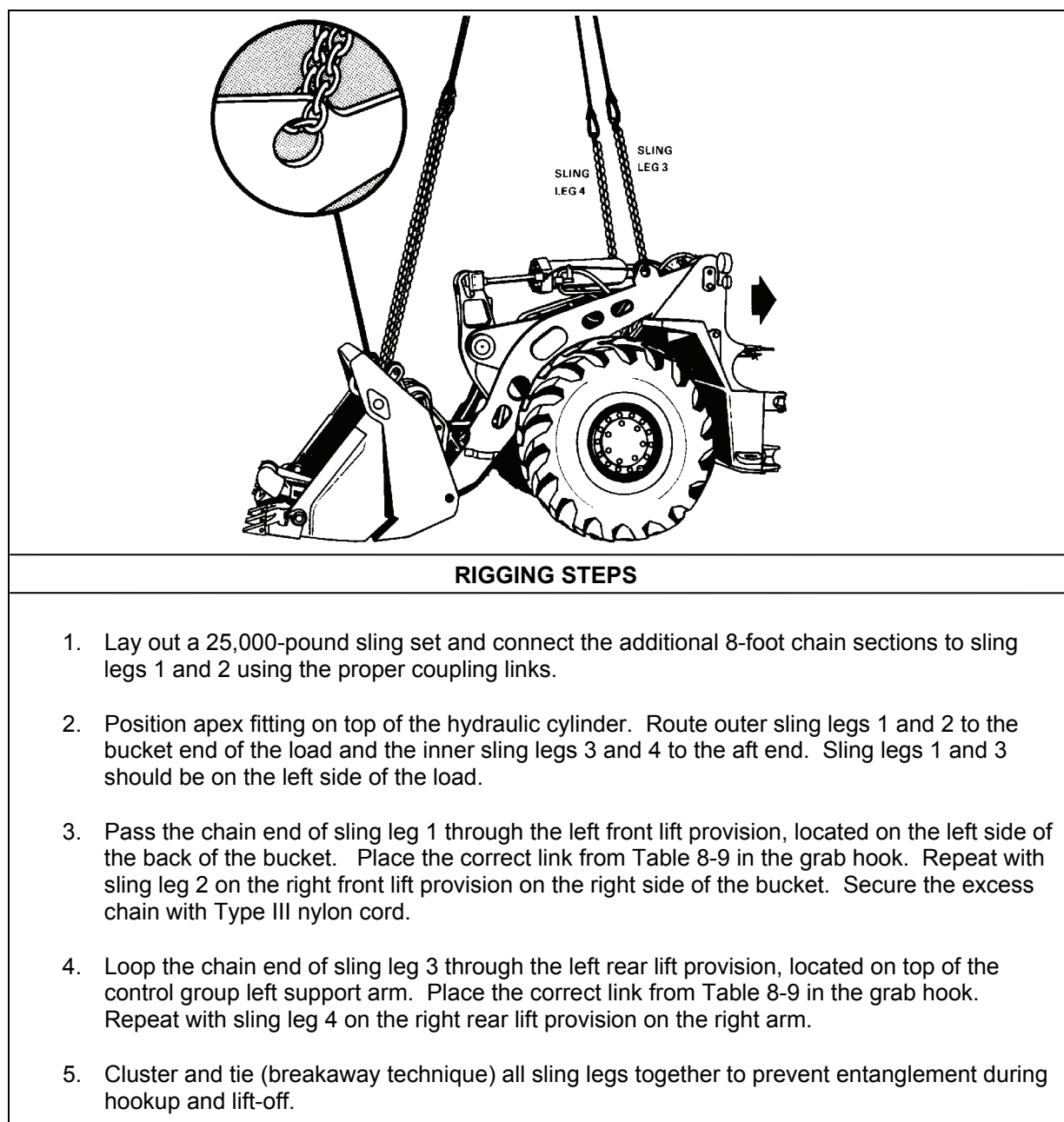
Figure 8-9a. 950BS Scoop Loader (Work Section)
