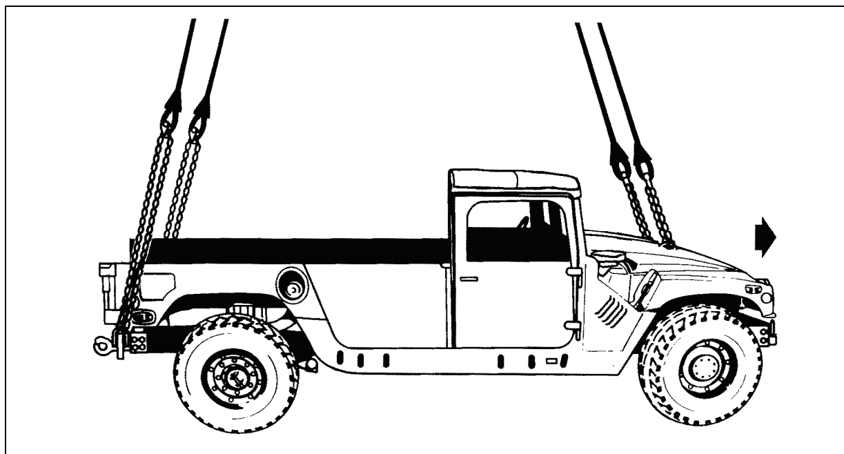
Figure 2-4. HMMWV Shelter Carriers without Shelter
