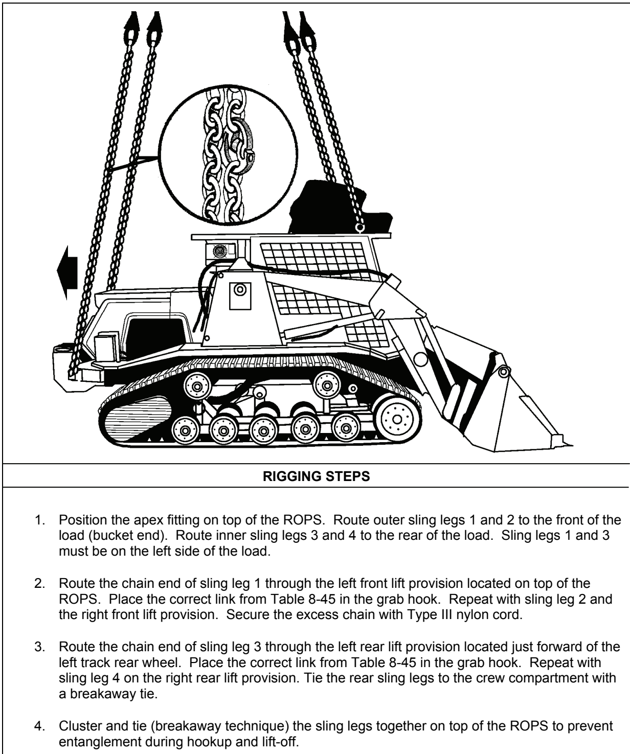
Figure 8-45. All-Purpose Remote Transport System Vehicle
