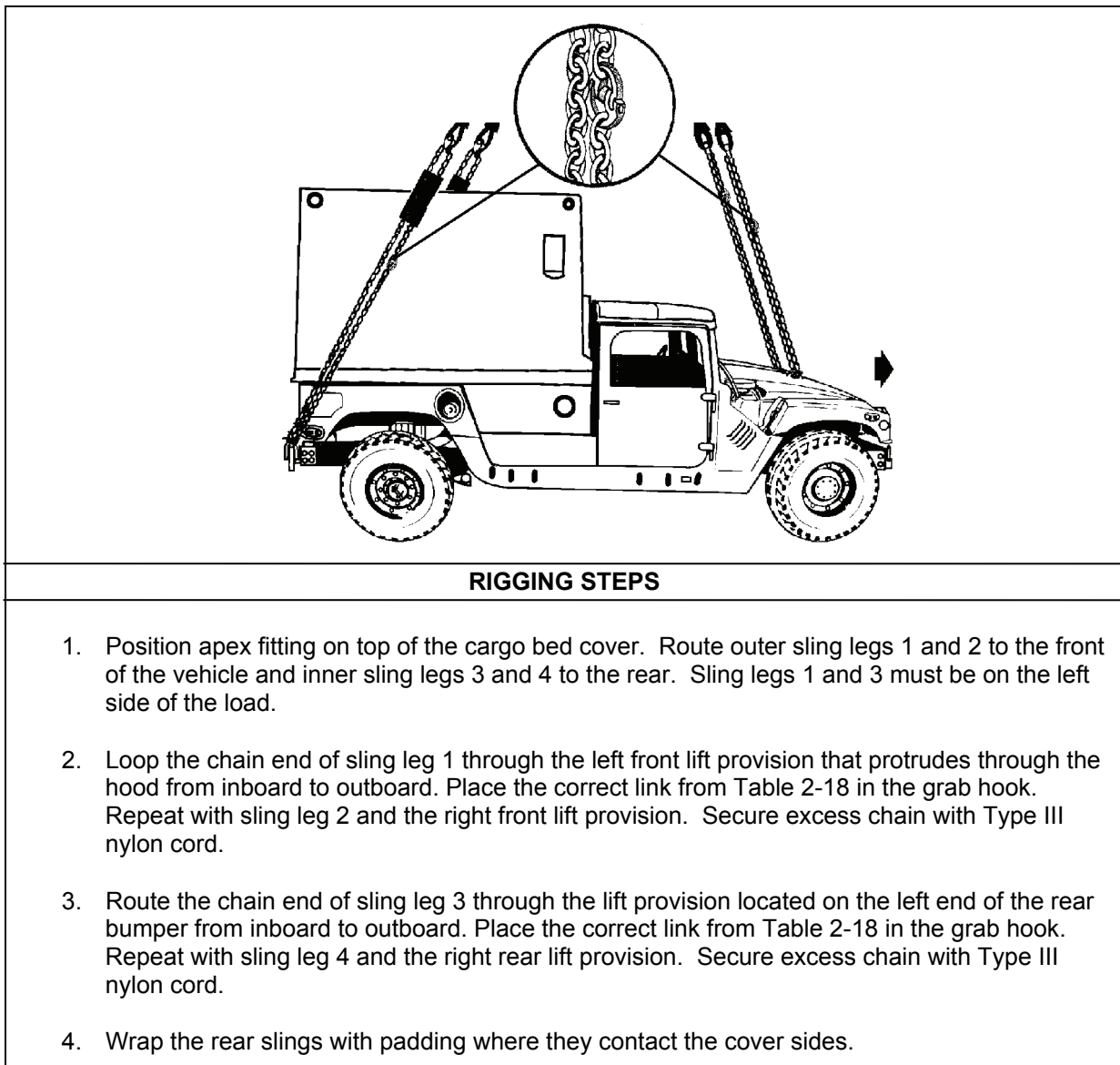
Figure 2-17. M1097 with Fiberglass Cargo Bed Cover
