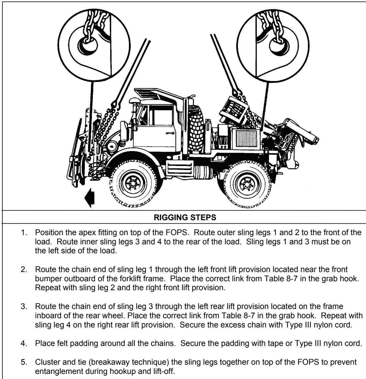
Figure 8-7. High Mobility Materiel Handler
