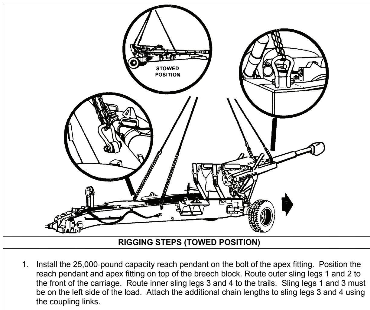
Figure 6-11. M198 155-MM Howitzer, Towed/Stowed
