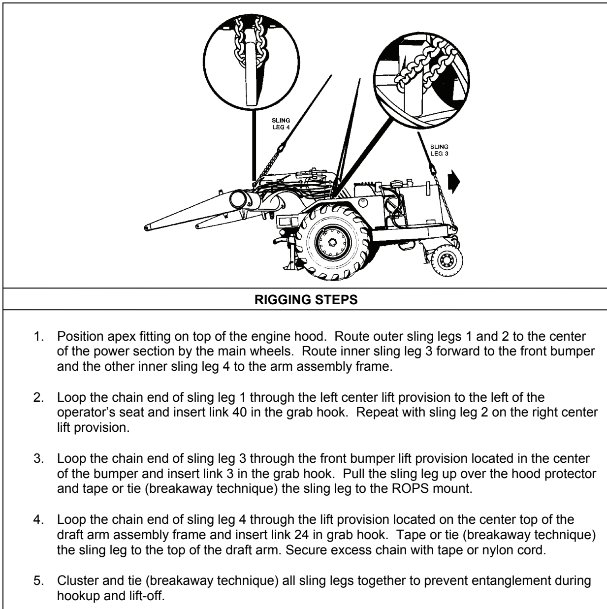
Figure 8-11b. 613BS Elevating Scraper (Power Section)
