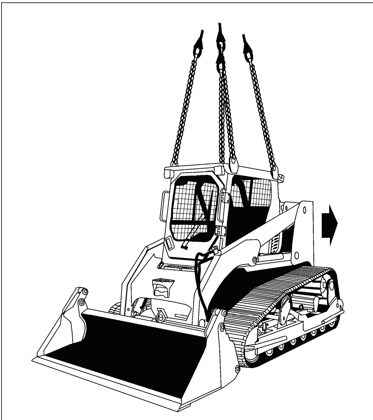
Figure 8-42. 277-Multi-Terrain Loader
