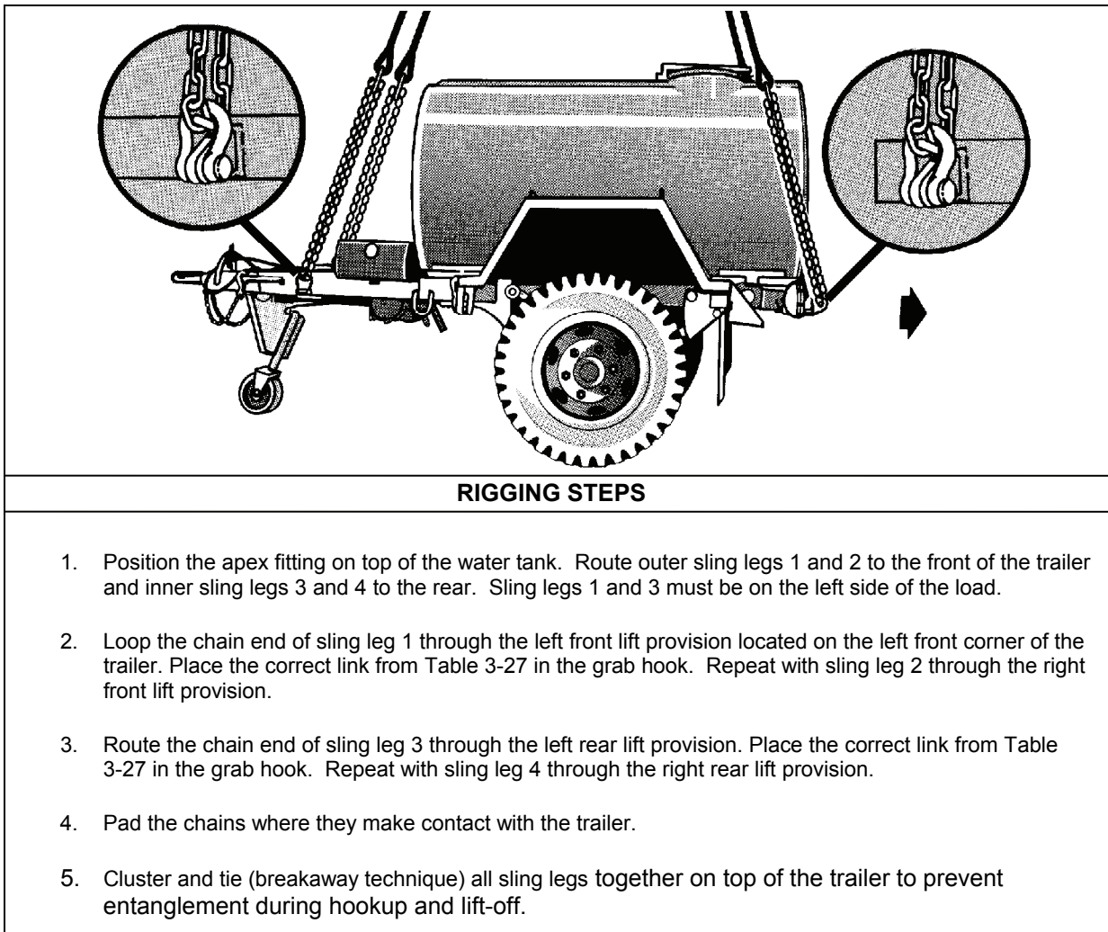
Figure 3-27. M1112 400 Gallon Water Trailer
