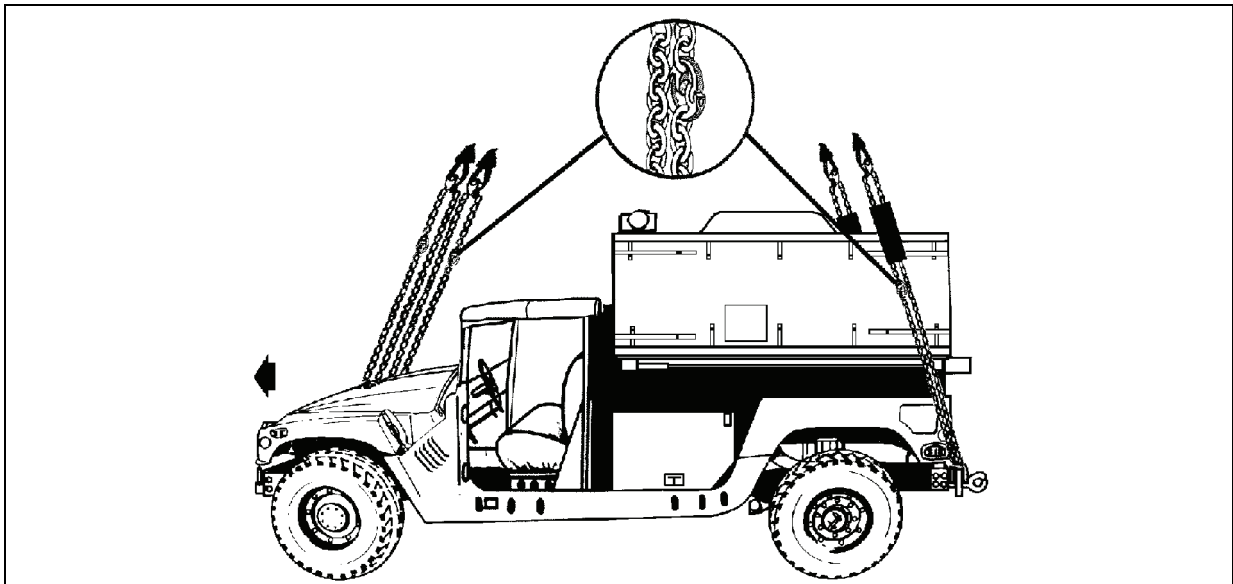
Figure 2-19. M1097A1 with Remote Landing Site Tower
