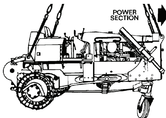
Figure 8-2a. D5B Tractor, Dozer, Track Section (Continued)
