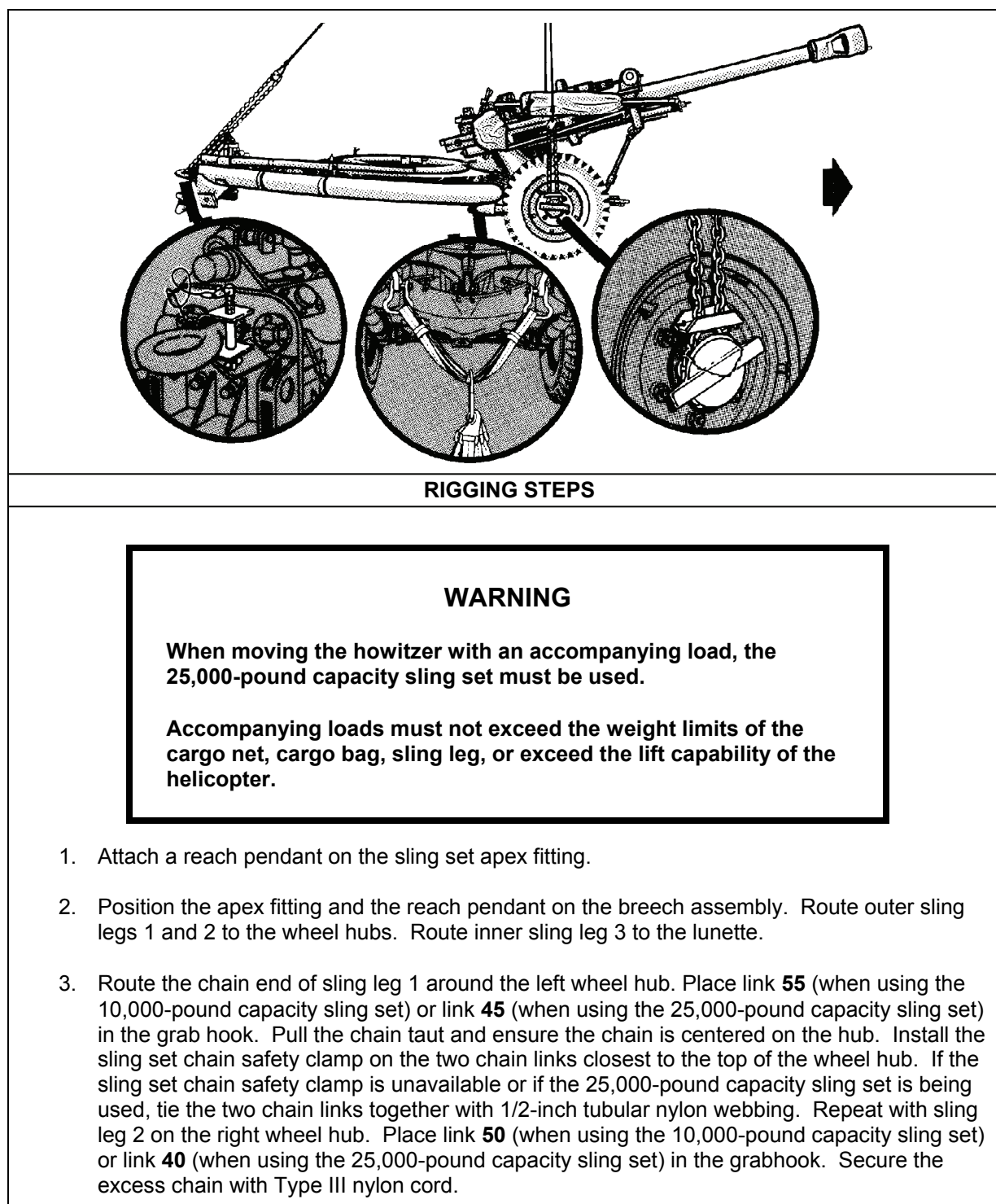
Figure 6-8. M119/M119A2 105-MM Howitzer, Forward/Firing Position
