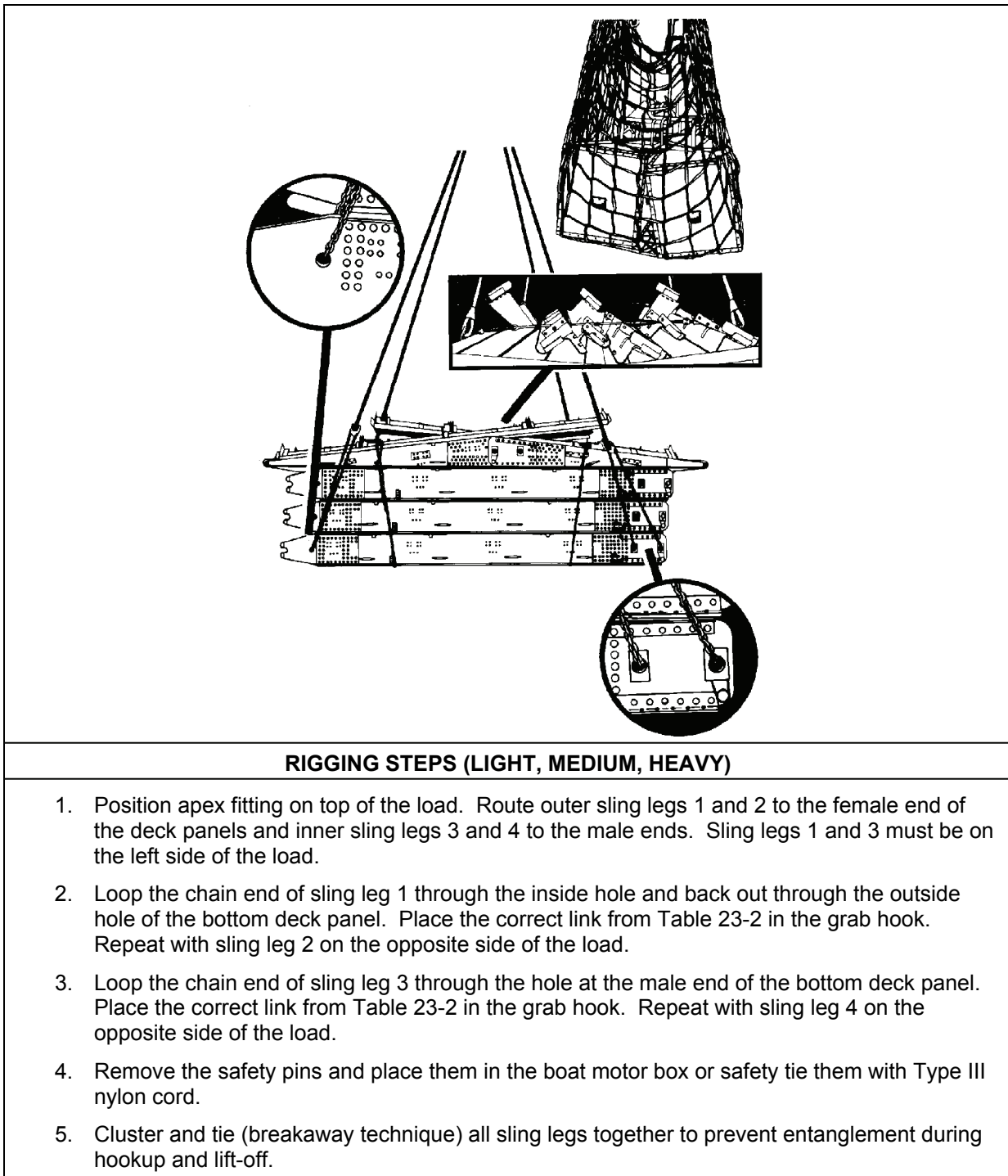
Figure 23-2. Light Tactical Floating Raft Bridge (Continued)
