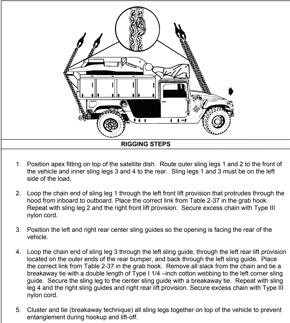
Figure 2-36. M1113 with Tactical Super High Frequency Satellite Terminal
