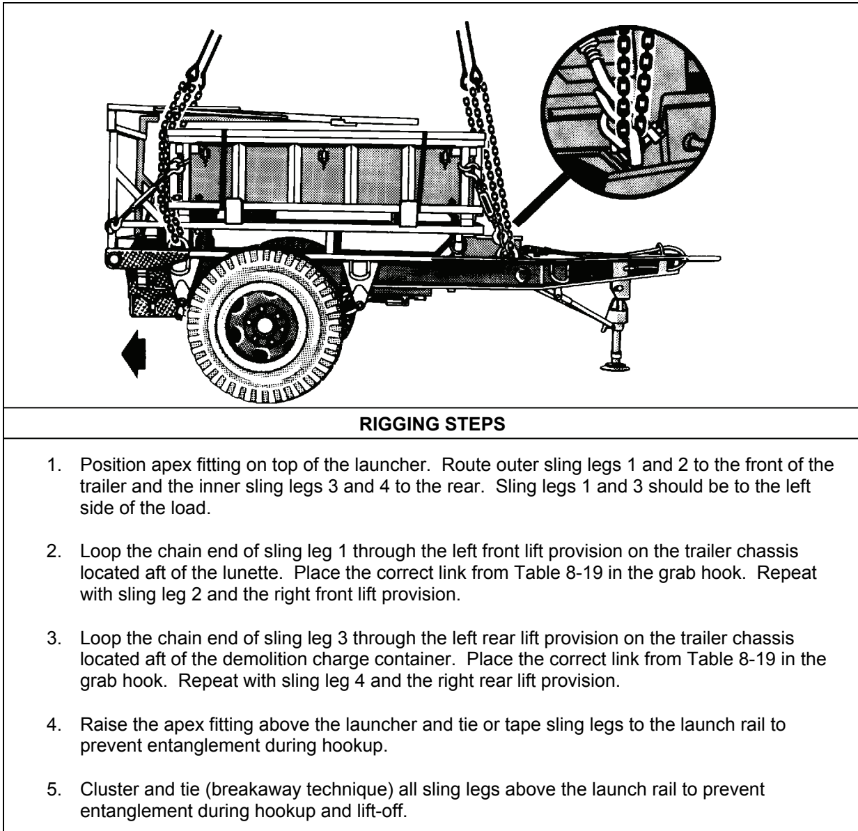
Figure 8-19. Mk155 Launcher on M200A1 or Mobile-Trac System Trailer
