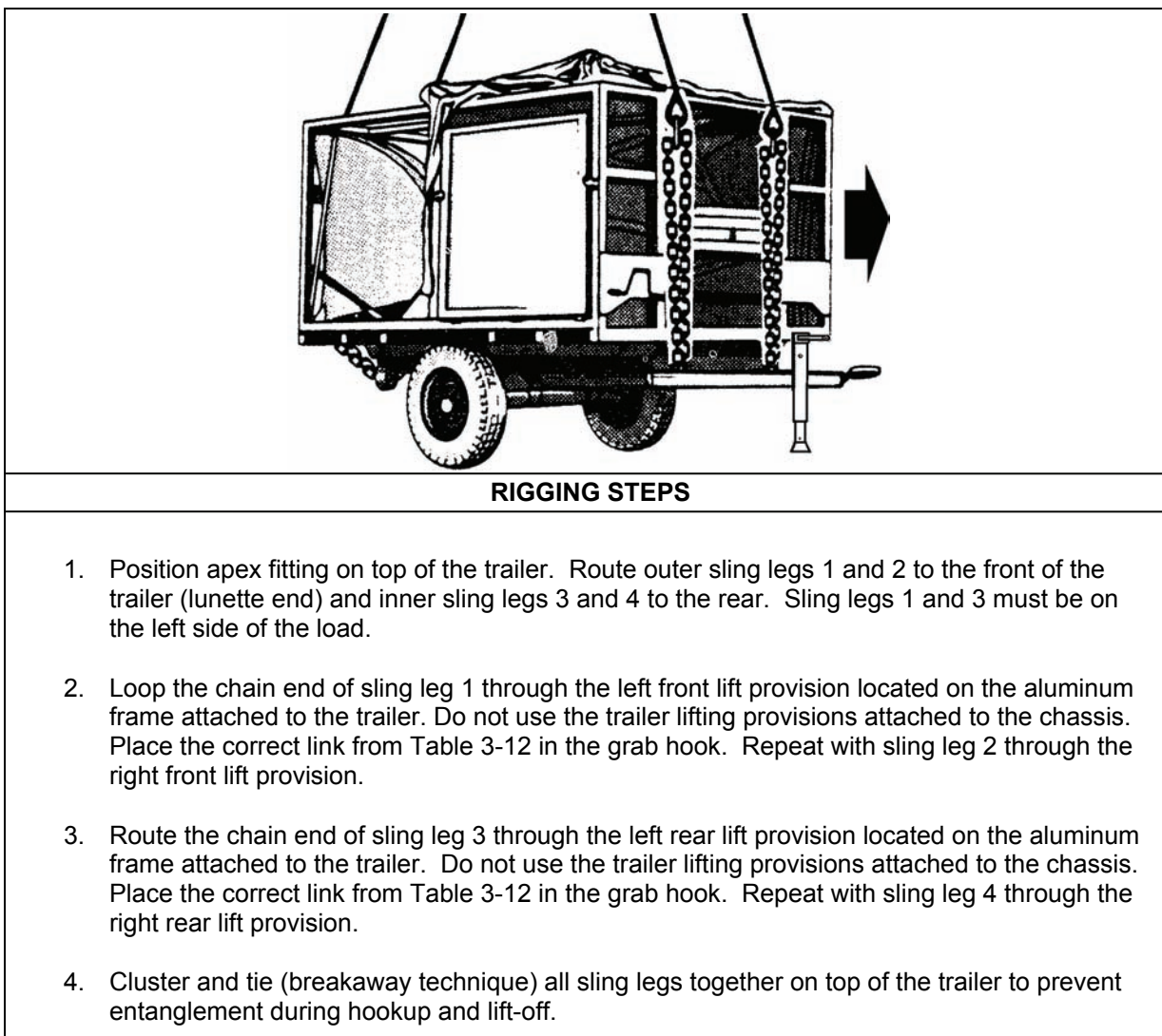
Figure 3-12. M116A2 Trailer with Antenna Groups, AS-3954/TRC (2 each)
