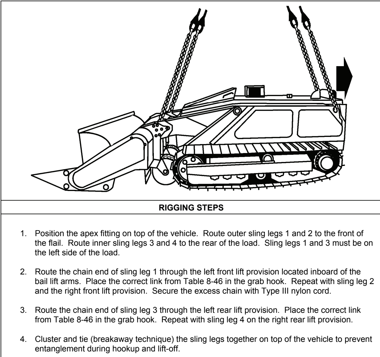
Figure 8-46. M4 Robotic Mine Flail
