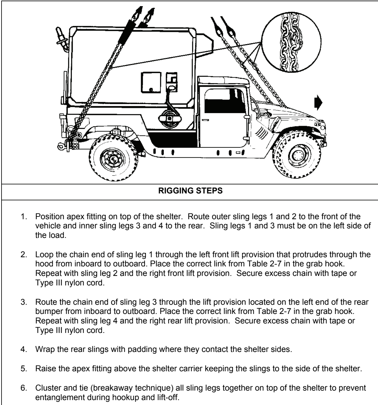
Figure 2-7. Downsized Direct Support Section Mounted on the M1037
