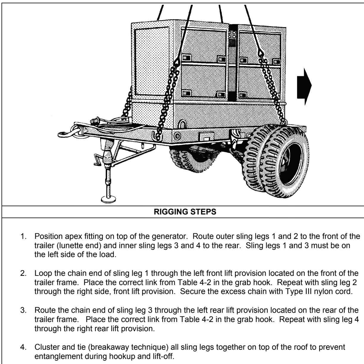
Figure 4-2. M200A1 Trailer-Mounted Power Units, Generators, and Power Plants
