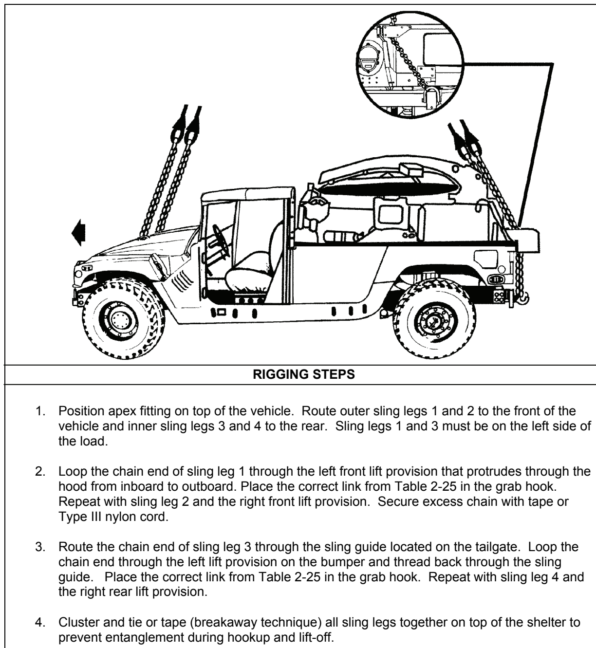
Figure 2-24. M1097A2 with Secure Mobile Anti-Jam Tactical Terminal Pallet
