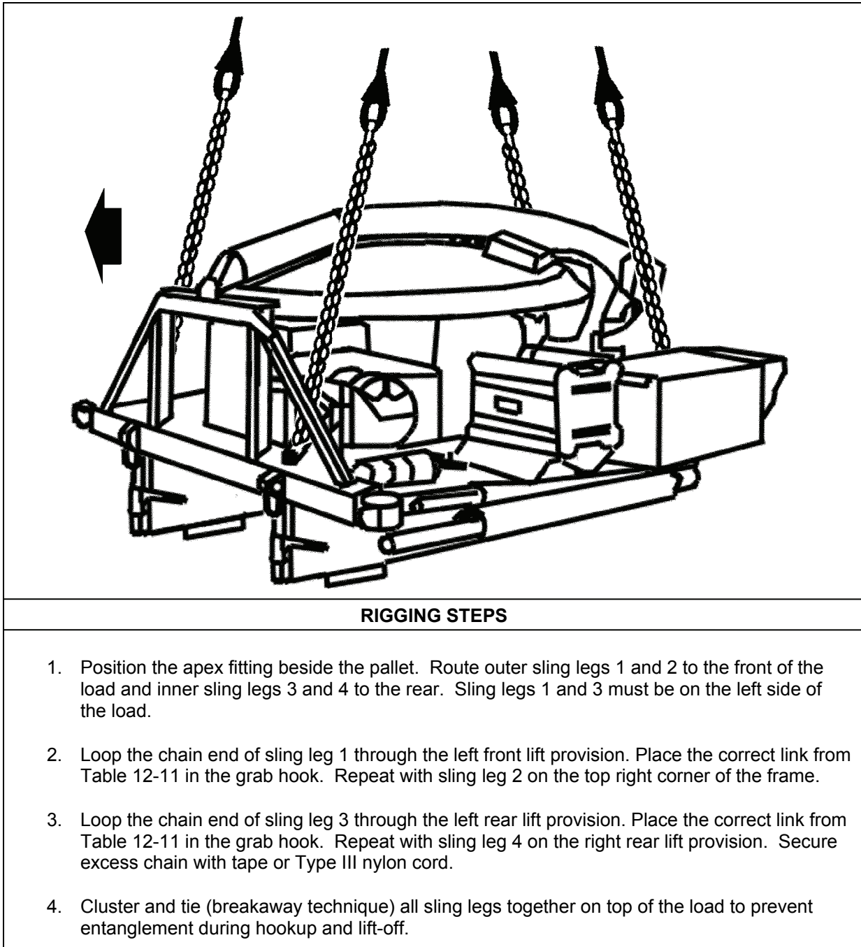
Figure 12-11. Secure Mobile Anti-Jam Reliable Tactical Terminal Pallet
