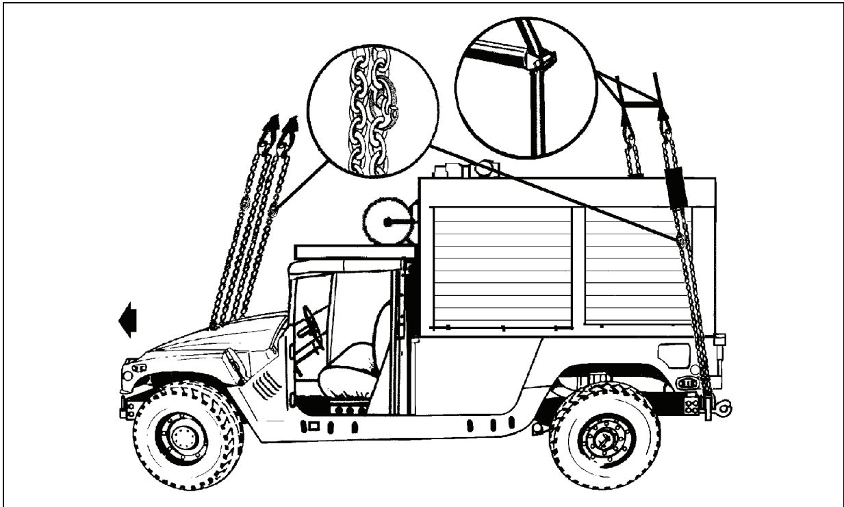
Figure 2-18. M1097 with Contact Maintenance Truck, Heavy
