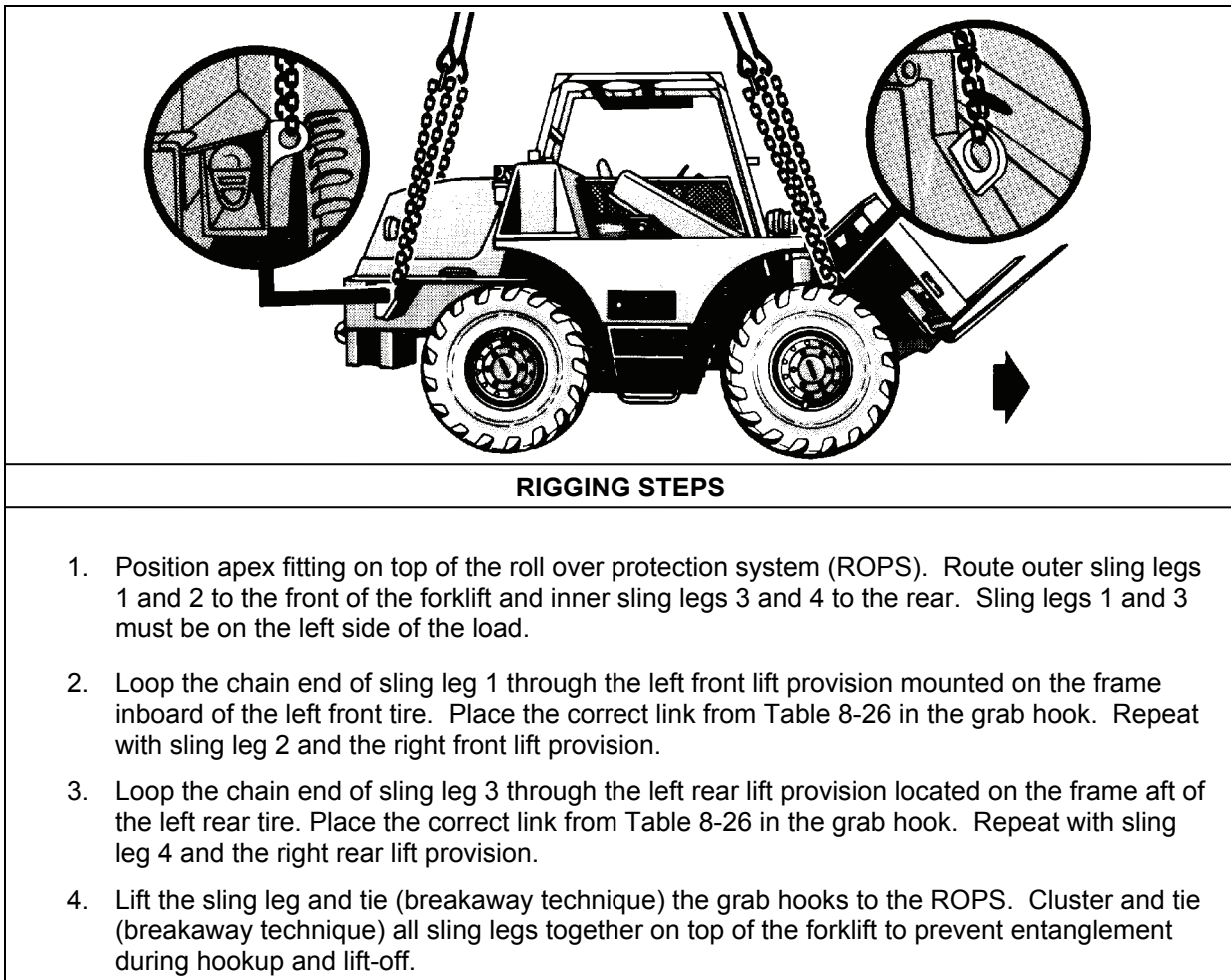
Figure 8-26. Truck, Forklift, MC-6000
