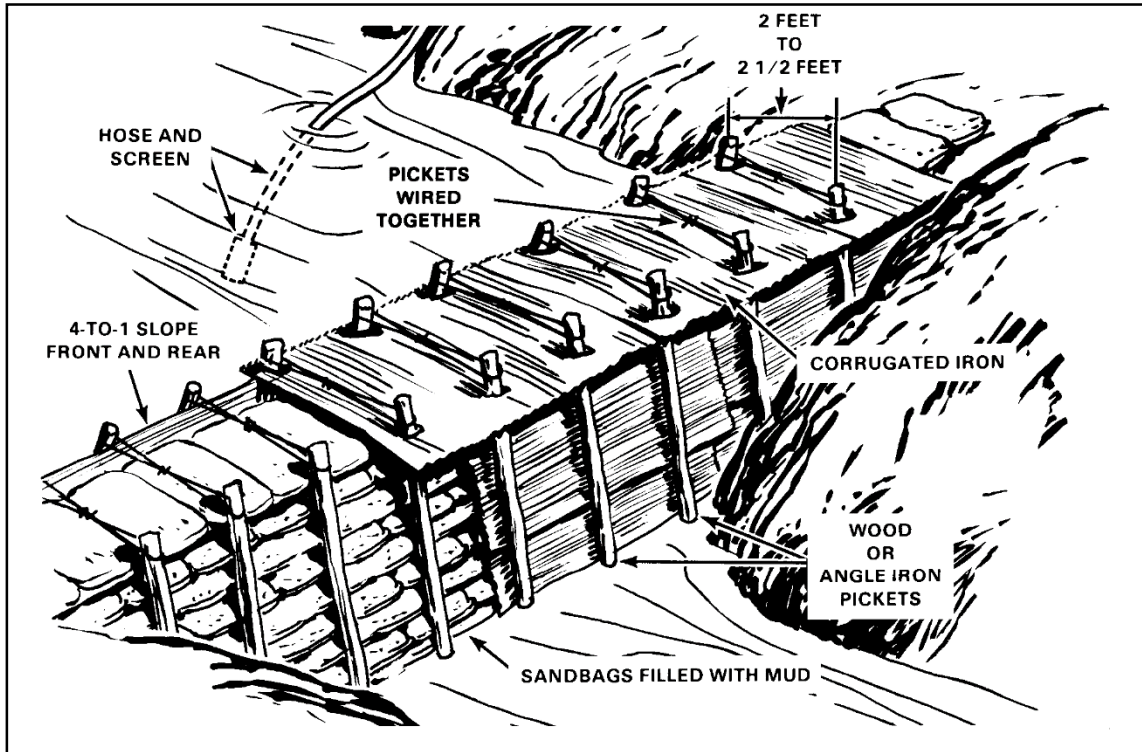
Figure 3-6. Improvised dam
