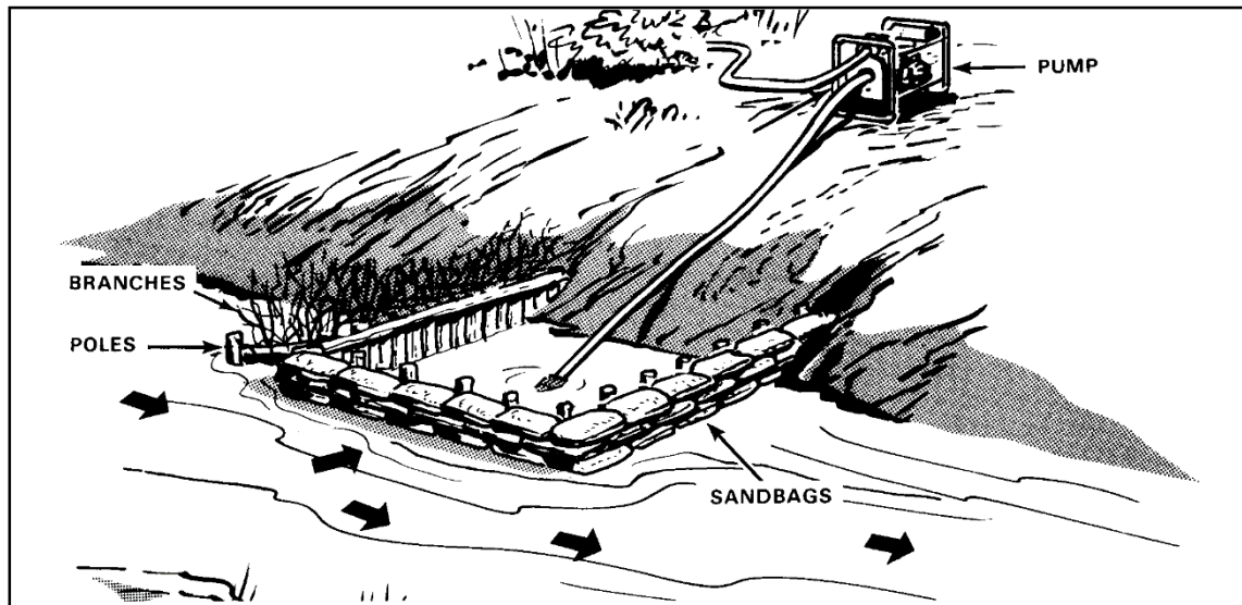
Figure 3-7. Baffle dam
