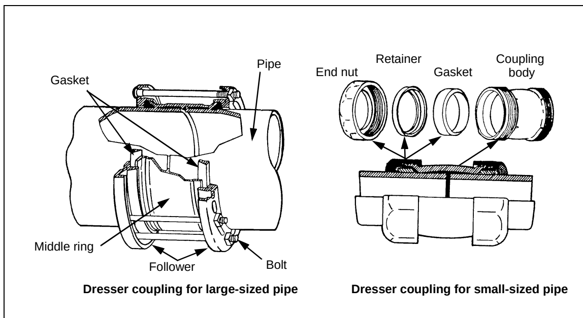
Figure 10-2. Dresser Couplings
