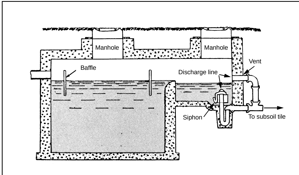
Figure 1-33. A Septic Tank With a Dosing Siphon
