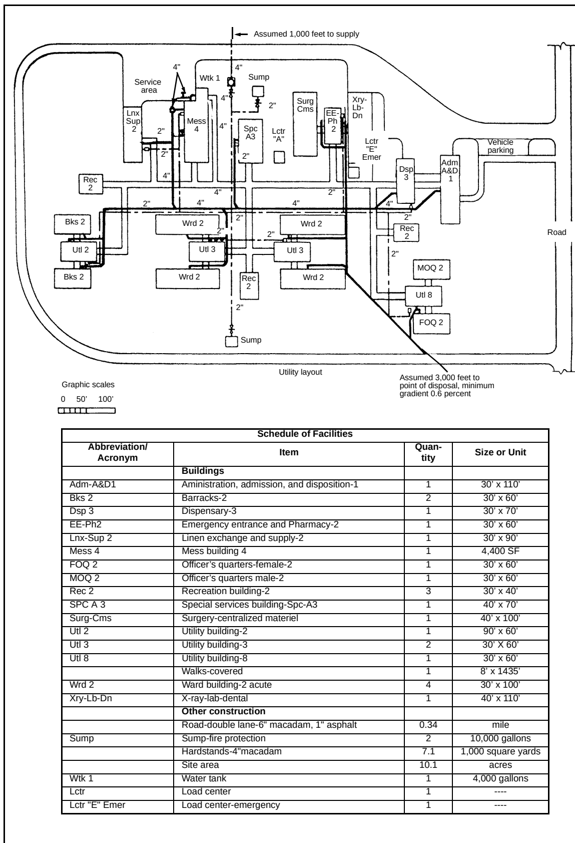
Figure B-1. Water Supply and Distribution System Plan
