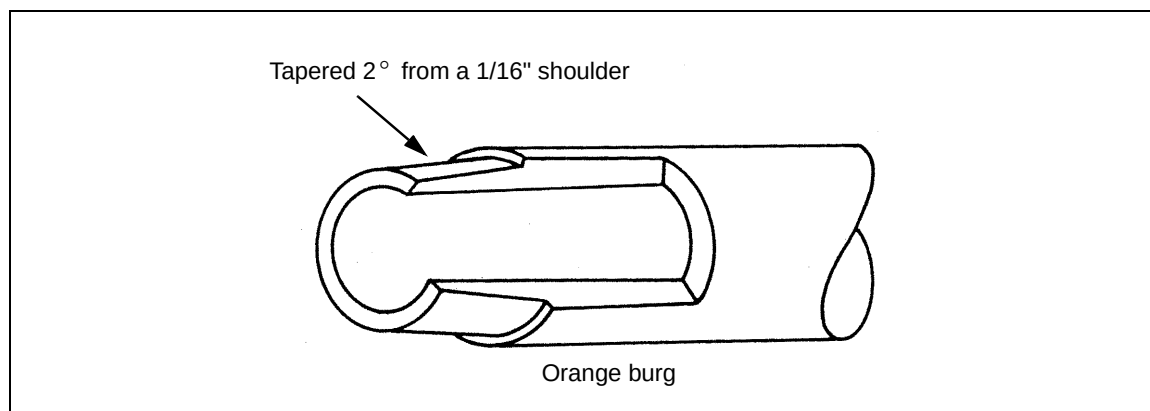
Figure 6-47. Bituminous-Fiber Pipe
