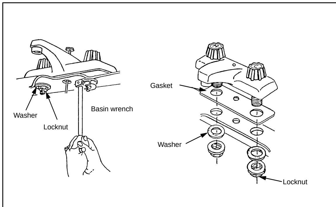
Figure 7-9. Faucet Installation
