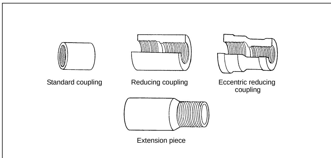
Figure 6-23. Couplings
