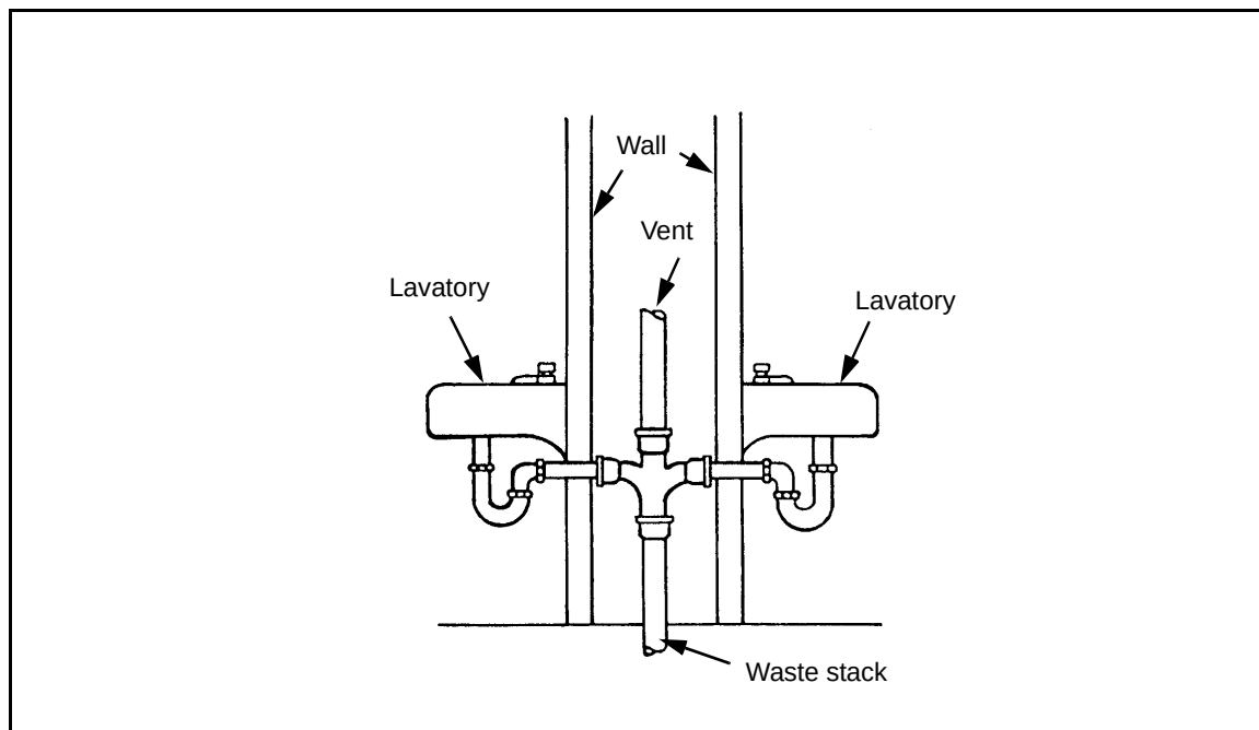
Figure 9-10. Common-Vented Fixtures
