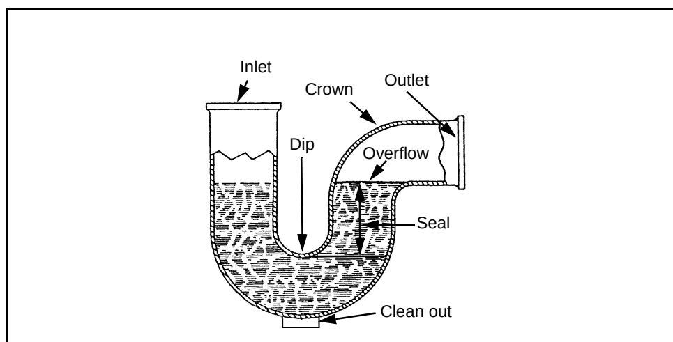
Figure 9-2. Trap Seal
