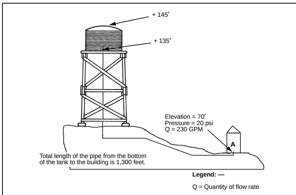
Figure E-4. Water Line, Design 1
