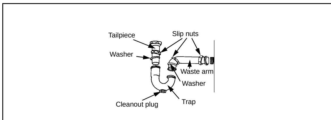
Figure 4-14. P-Trap Connection
