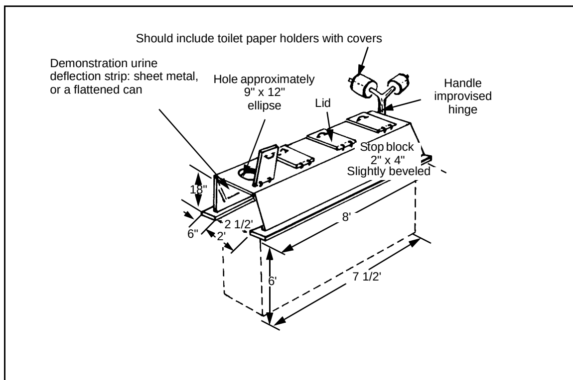
Figure 1-16. Deep-Pit Latrine
