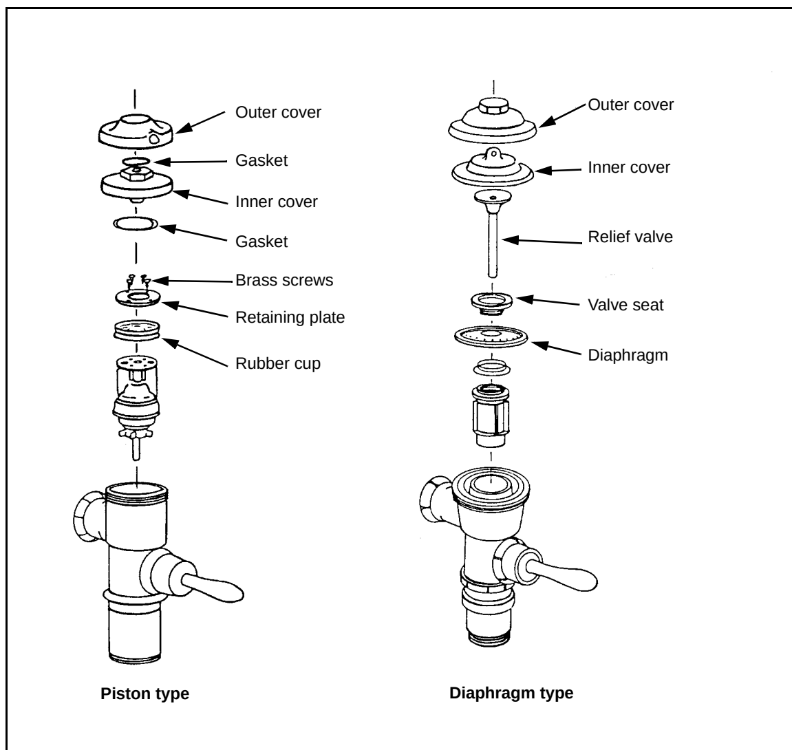
Figure 4-8. Flushometer Repairs
