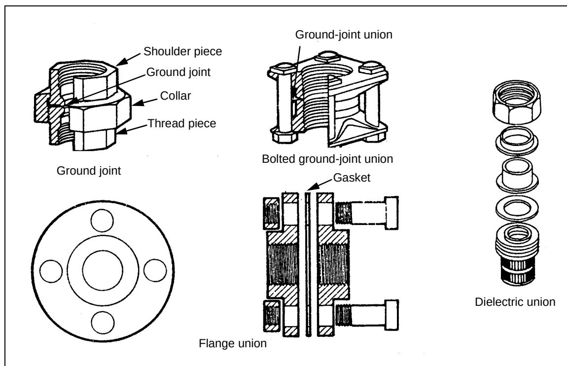
Figure 6-24. Unions
