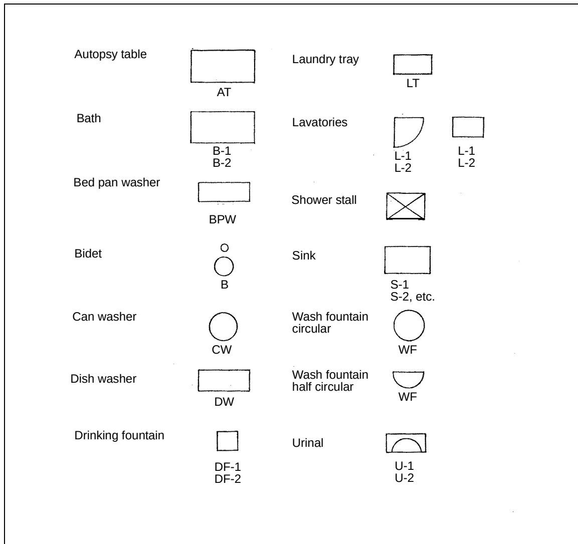
Figure B-13. Plumbing Symbols
