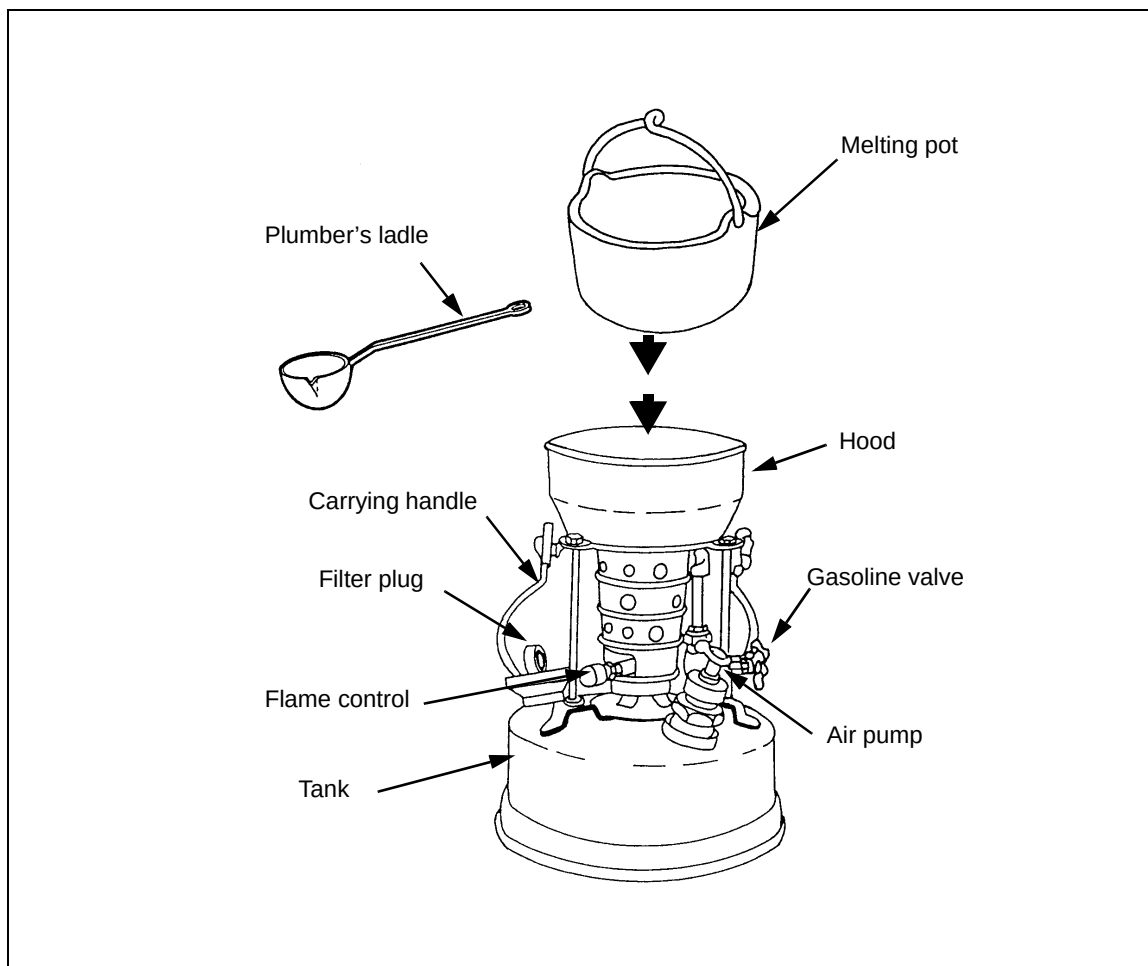
Figure 6-15. Lead-Melting Furnace
