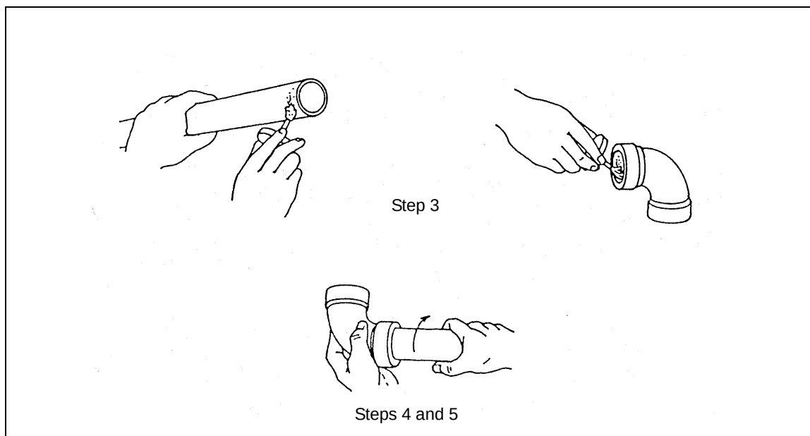
Figure 6-45. Rigid Plastic Pipe Joint
