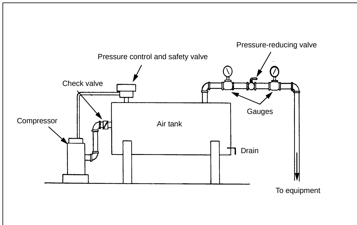
Figure 10-1. Air-Compressor Tank
