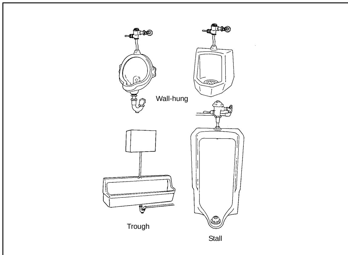
Figure 4-19. Urinals
