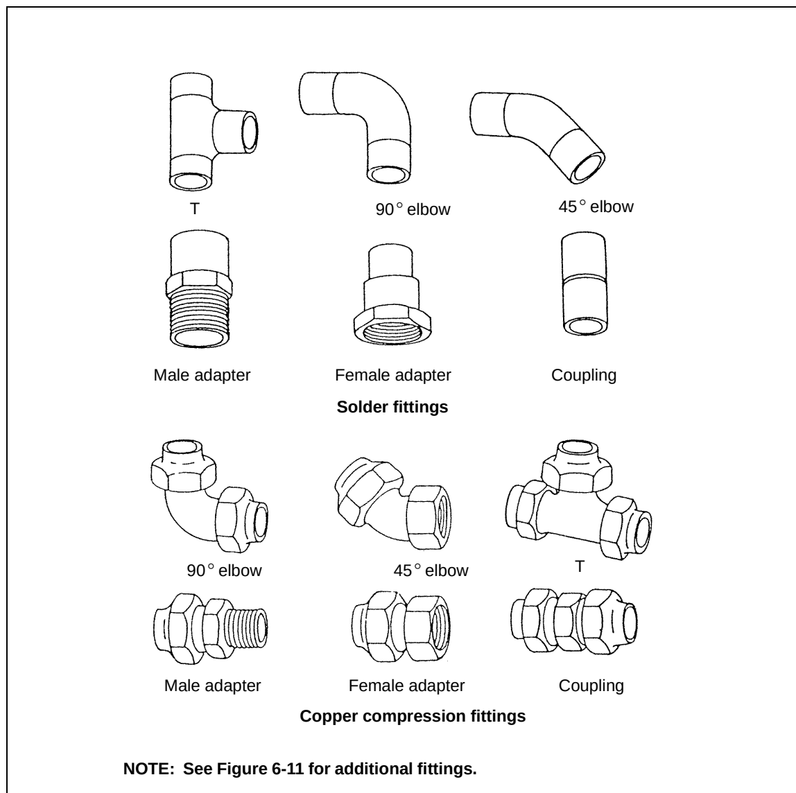
Figure 6-32. Copper-Tubing Fittings
