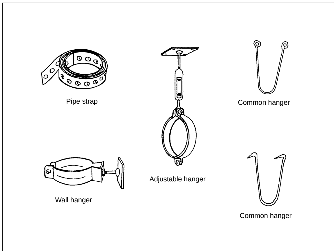
Figure 6-1. Pipe Hangers
