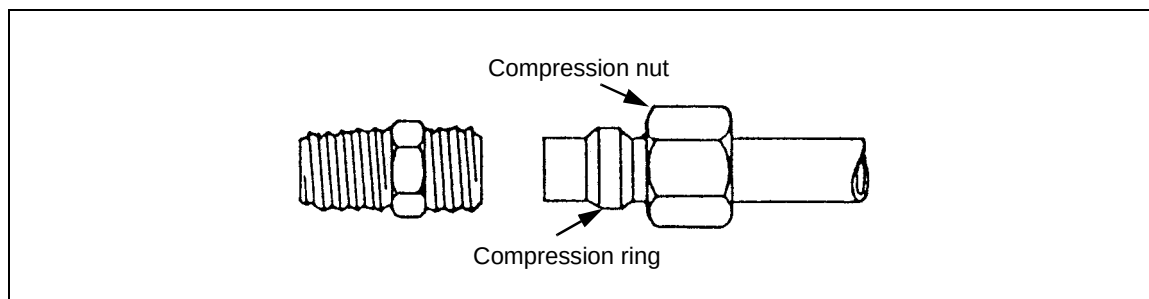
Figure 6-39. Mechanical-Compression Joint
