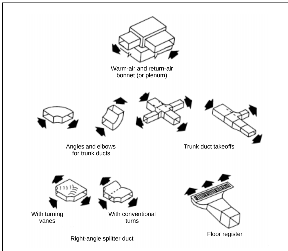
Figure 2-10. Rectangular Duct Connections
