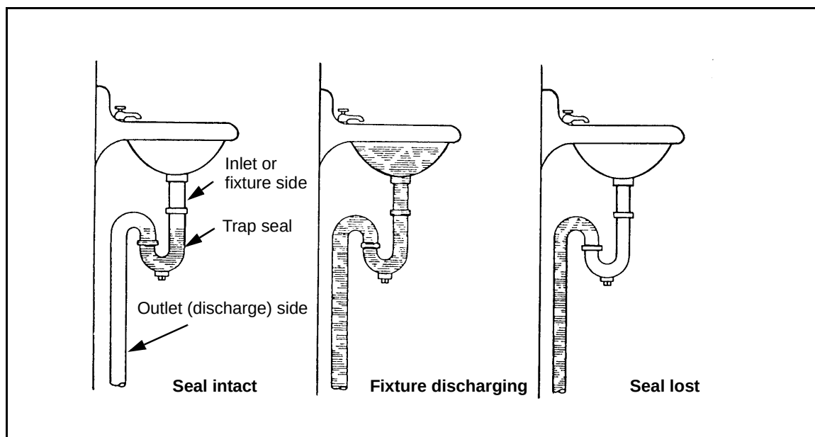
Figure 9-3. Direct Siphonage
