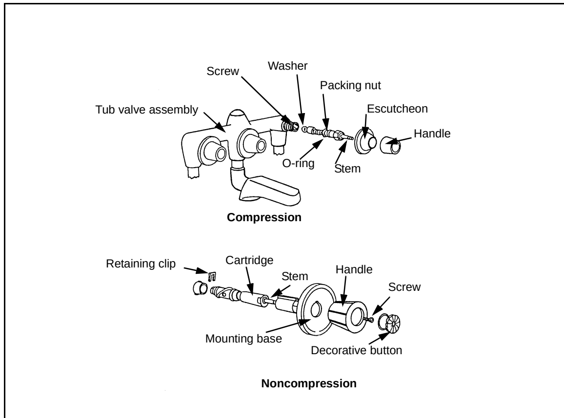
Figure 7-13. Bathtub Faucet Breakout
