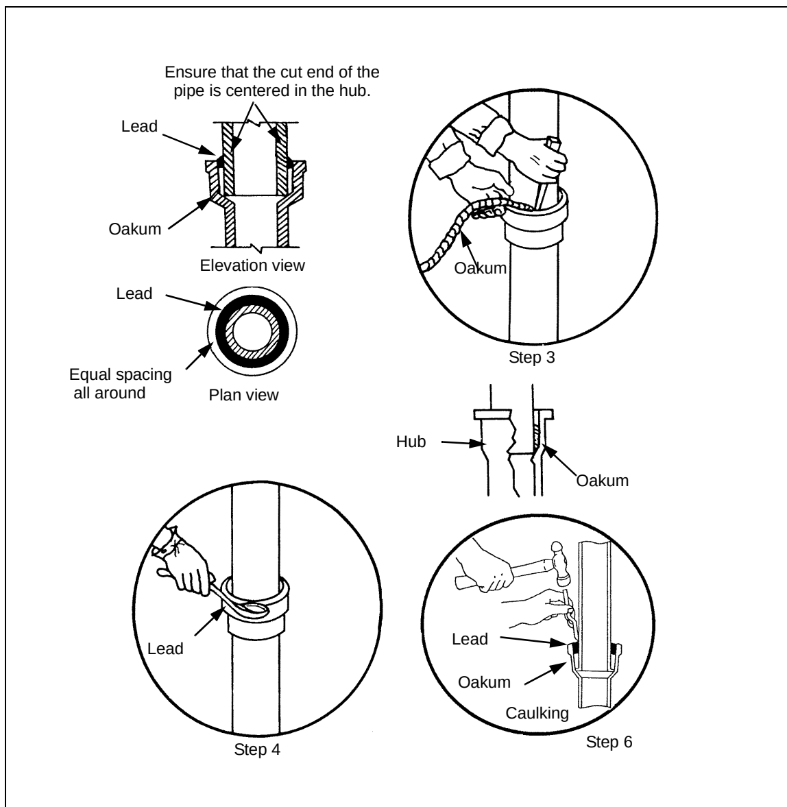
Figure 6-17. Vertical Lead Joint
