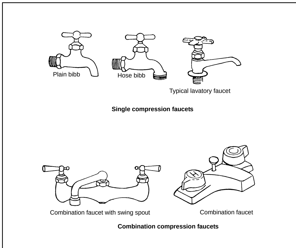
Figure 7-6. Compression Faucets
