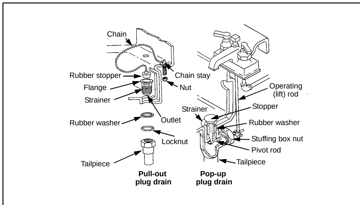
Figure 4-13. Drain-Plug Assembly
