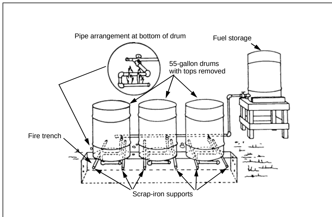
Figure 5-6. Vapor Burner
