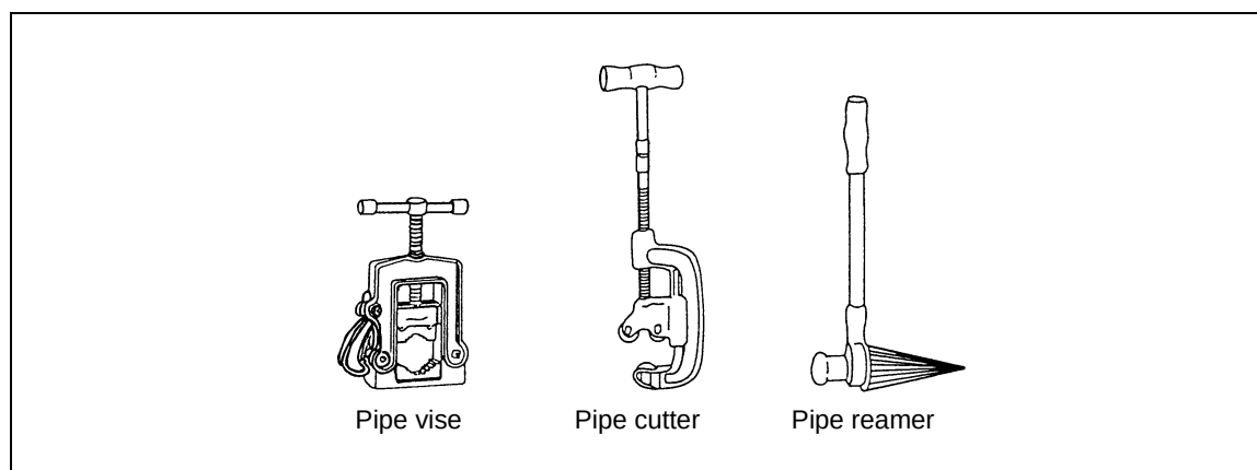
Figure 6-26. Steel-Pipe Tools
