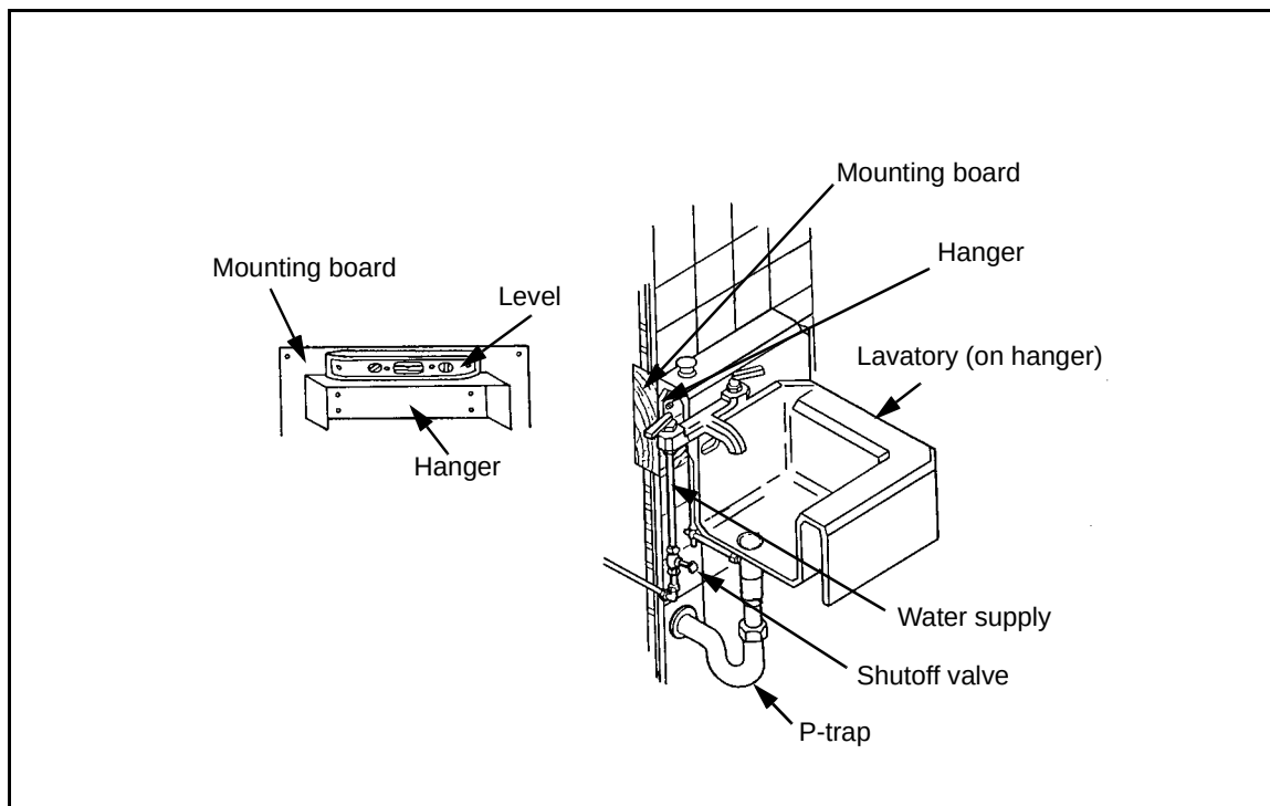
Figure 4-12. Wall-Hung Lavatory Installation
