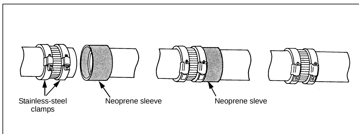
Figure 6-18. Hubless Joint
