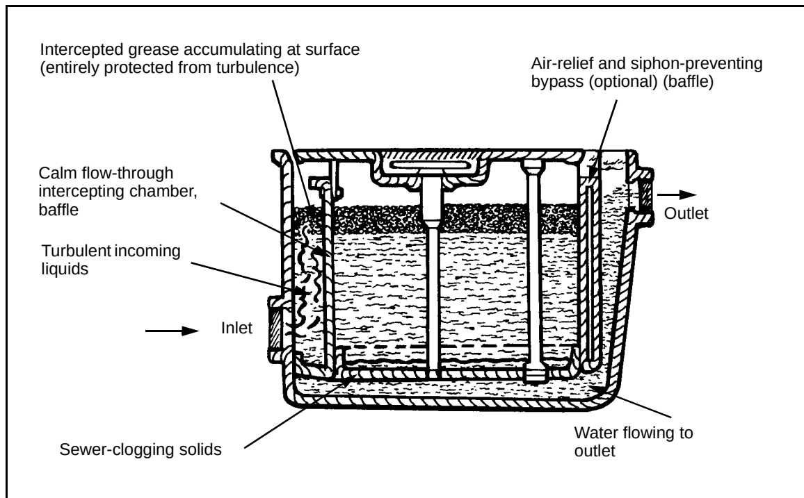
Figure 1-8. Grease Trap
