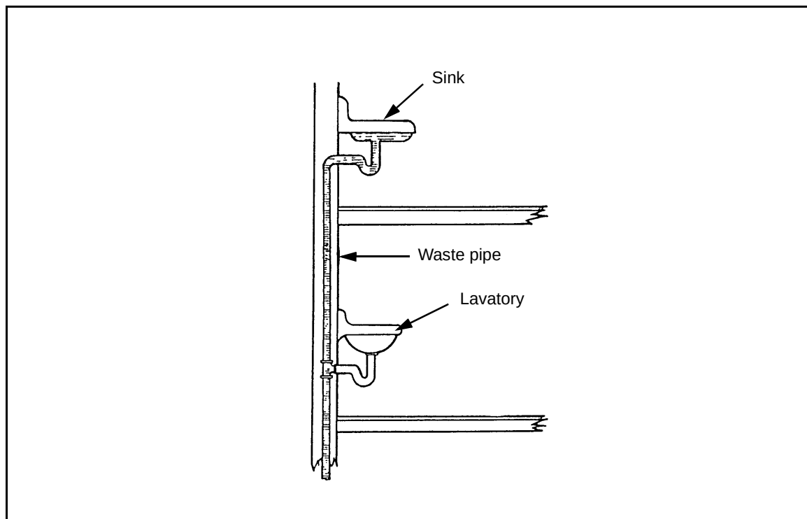
Figure 9-4. Indirect Siphonage
