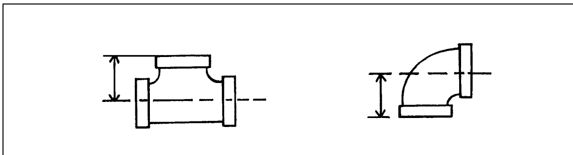
Figure 6-3. Fitting Dimension
