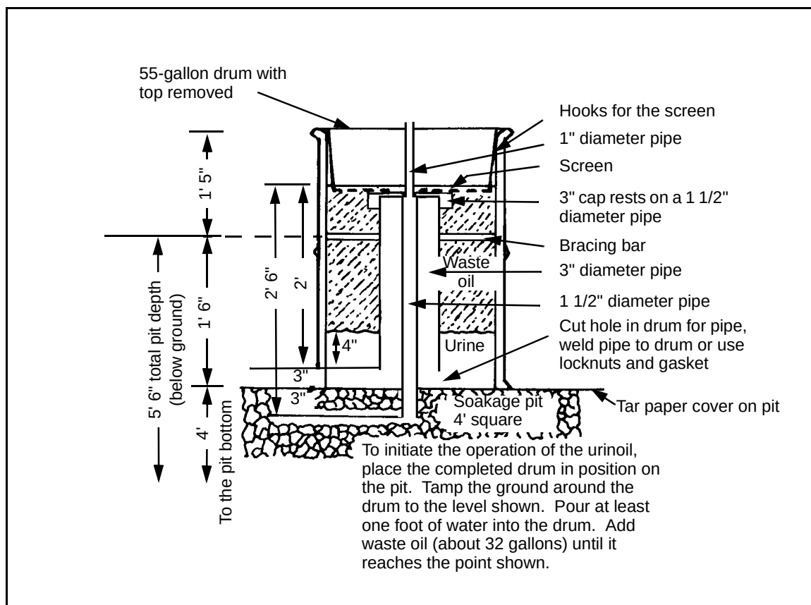
Figure 1-23. Urinal
