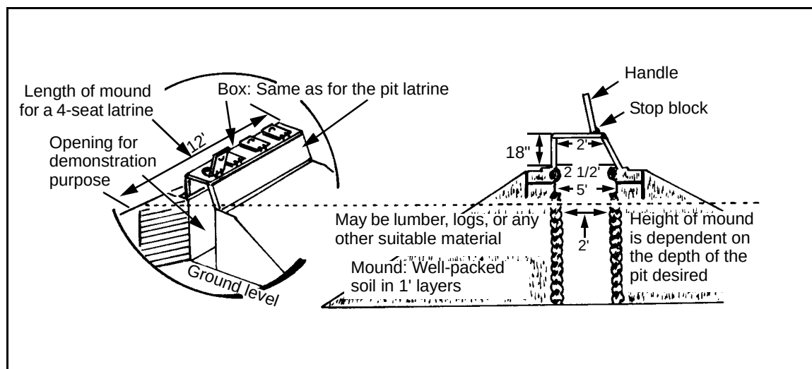
Figure 1-18. Mounded Latrine
