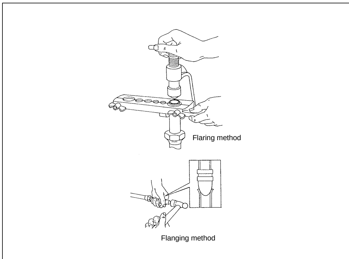
Figure 6-37. Flaring and Flanging Flexible Copper Tubing
