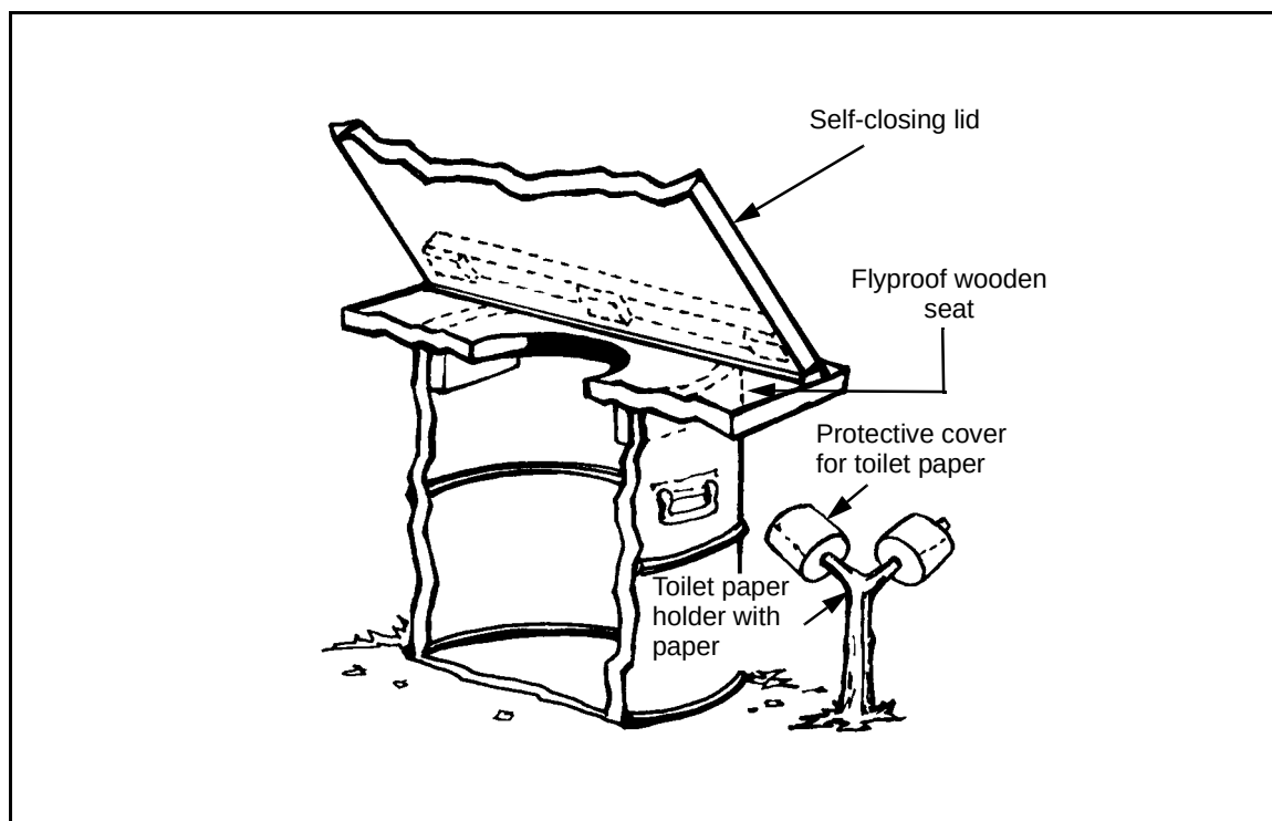
Figure 1-19. Burn-Out Latrine
