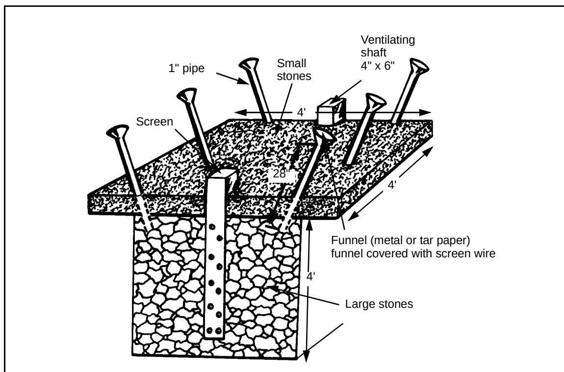
Figure 1-21. Urine Soakage Pit with Pipe Urinals
