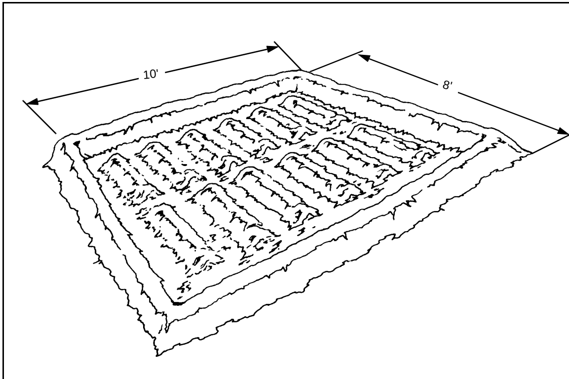
Figure 1-27. Evaporation Bed
