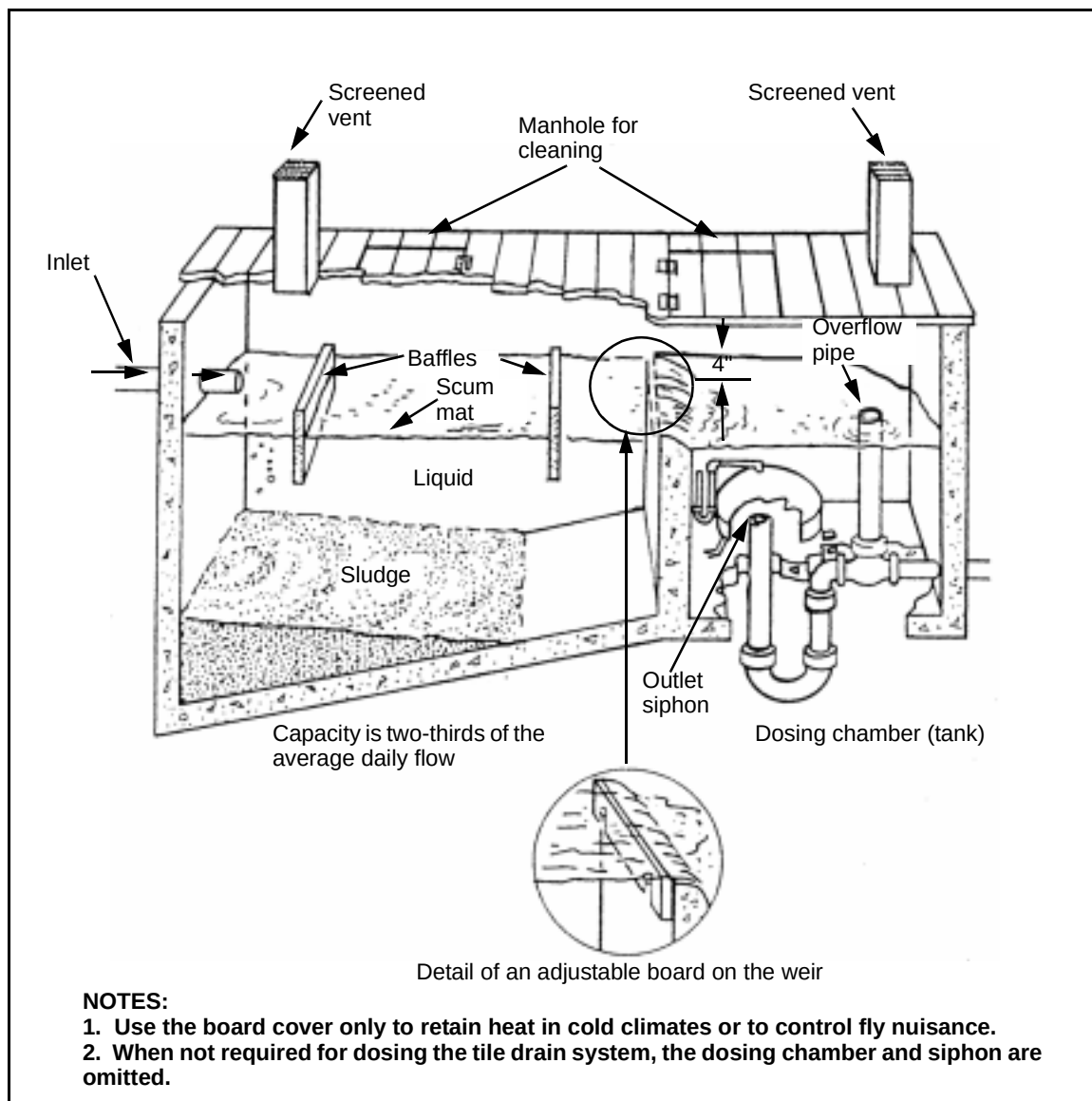
Figure 1-9. Septic Tank
