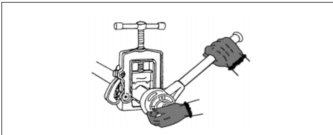
Figure 6-29. Threading Pipe
