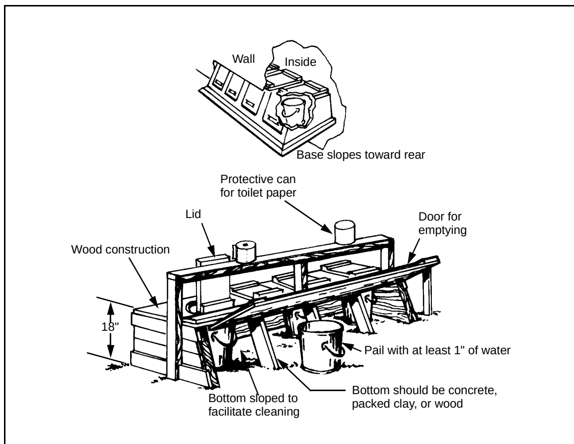
Figure 1-20. Pail Latrine
