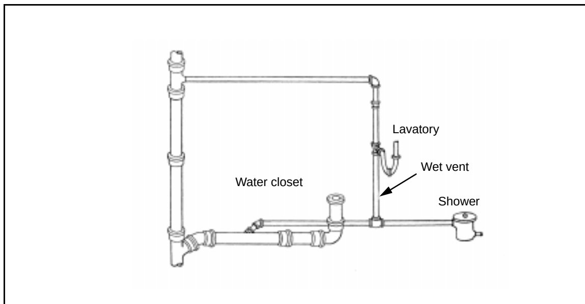
Figure 9-12. Group of Wet-Vent Fixtures
