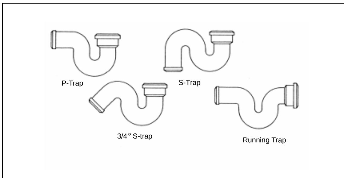
Figure 6-10. Cast-Iron Traps
