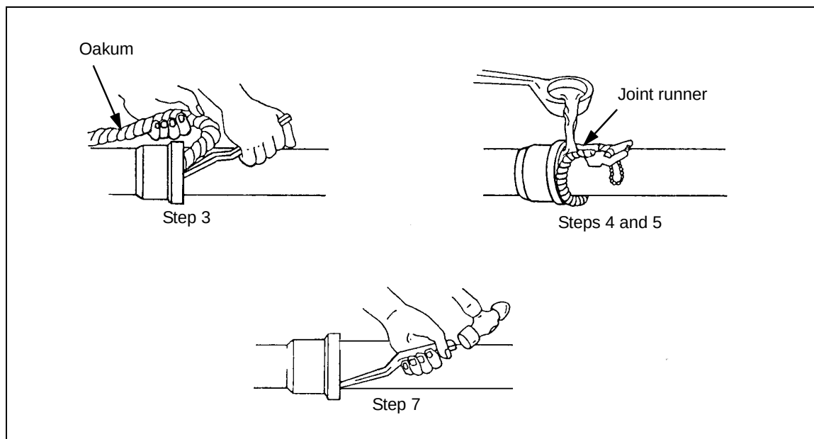
Figure 6-16. Horizontal Lead Joint
