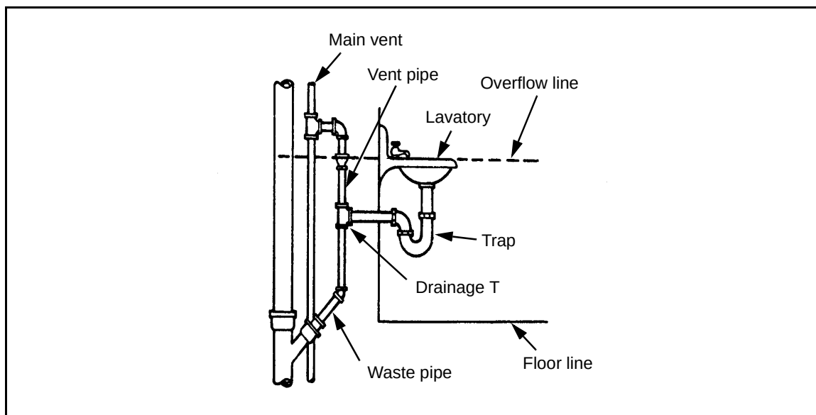
Figure 9-8. Single-Fixture Vent
