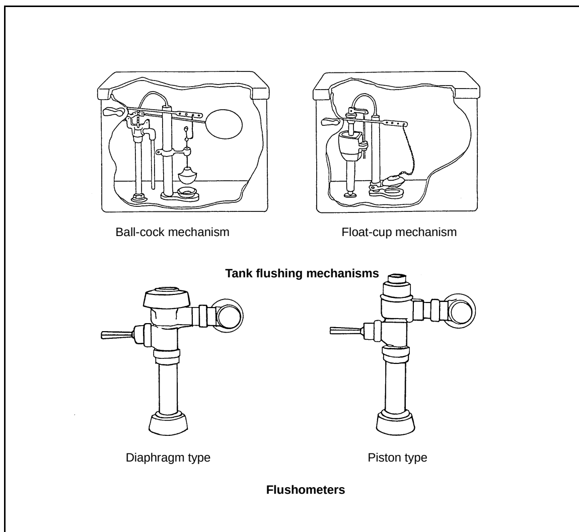
Figure 4-6. Flushing Mechanisms
