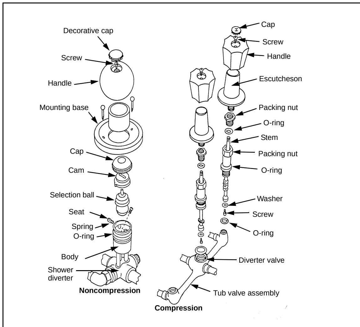
Figure 7-12. Bathtub and Shower Faucet Breakout
