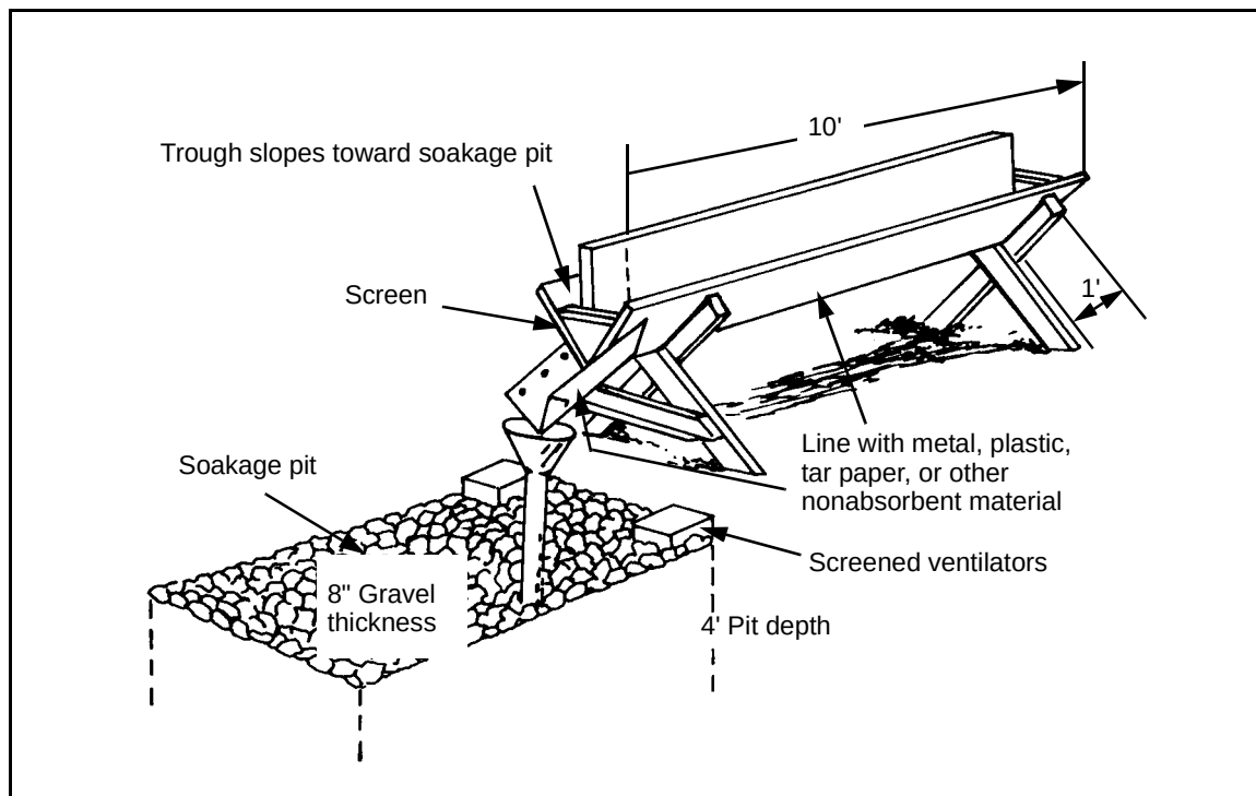
Figure 1-22. Trough Urinal
