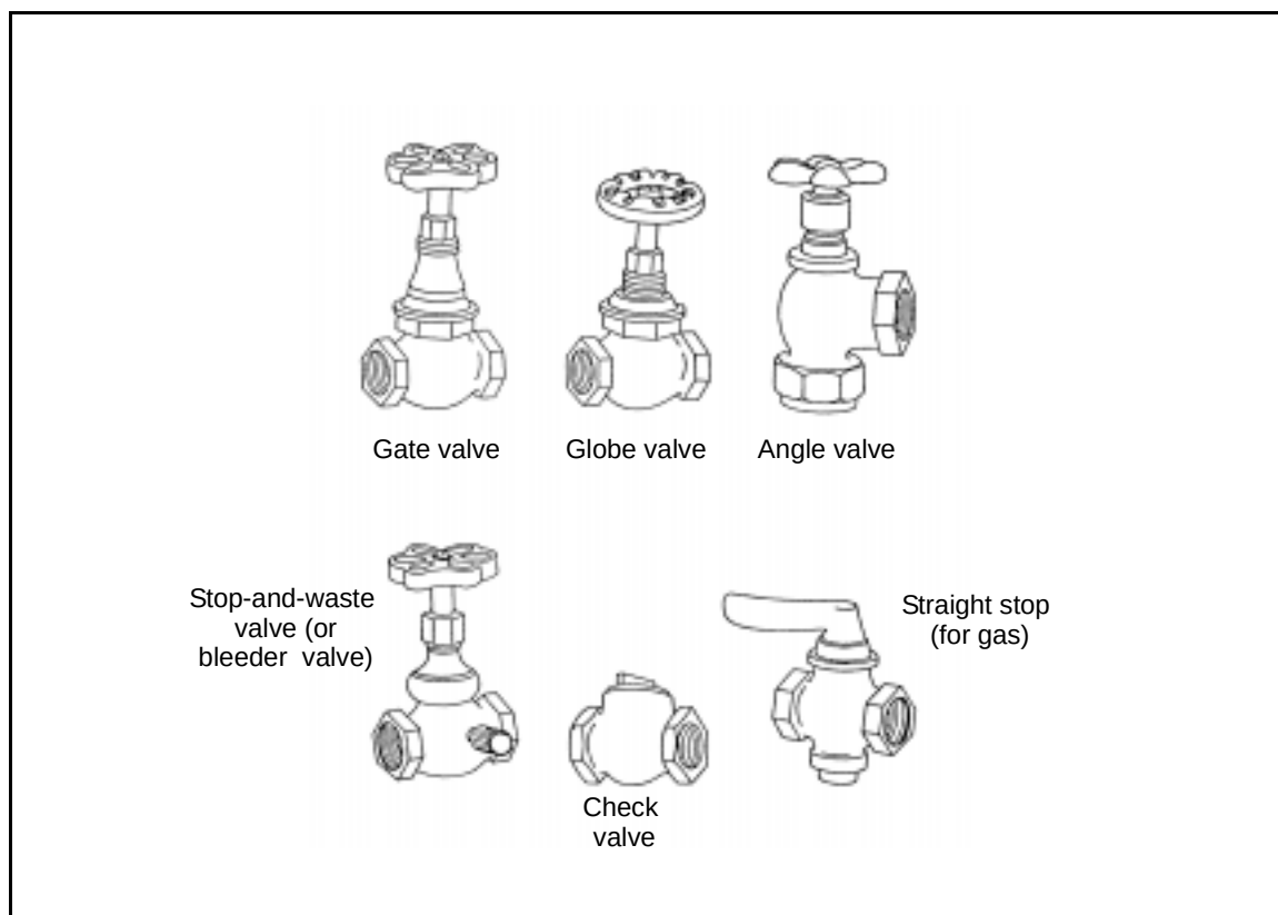
Figure 7-1. Valves
