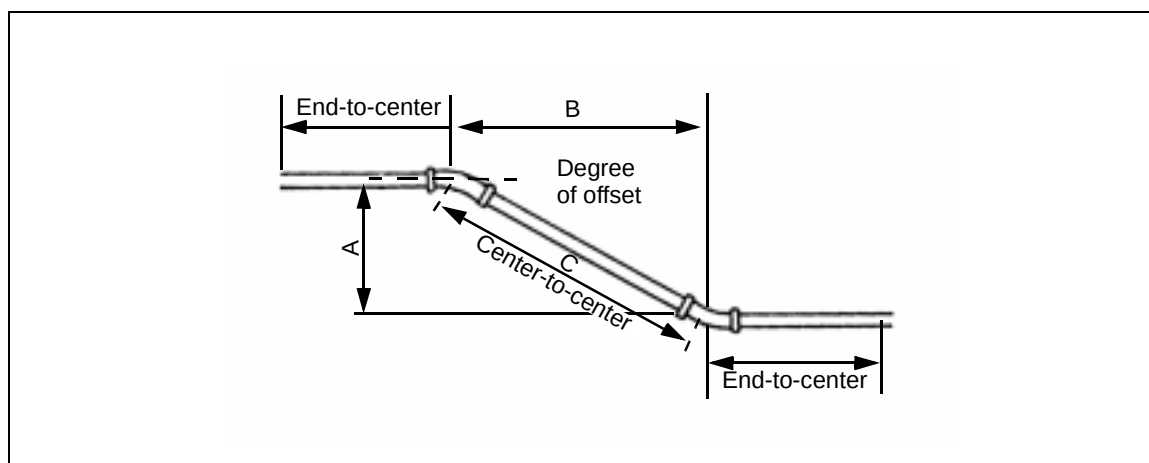
Figure 6-5. Offset Measurement
