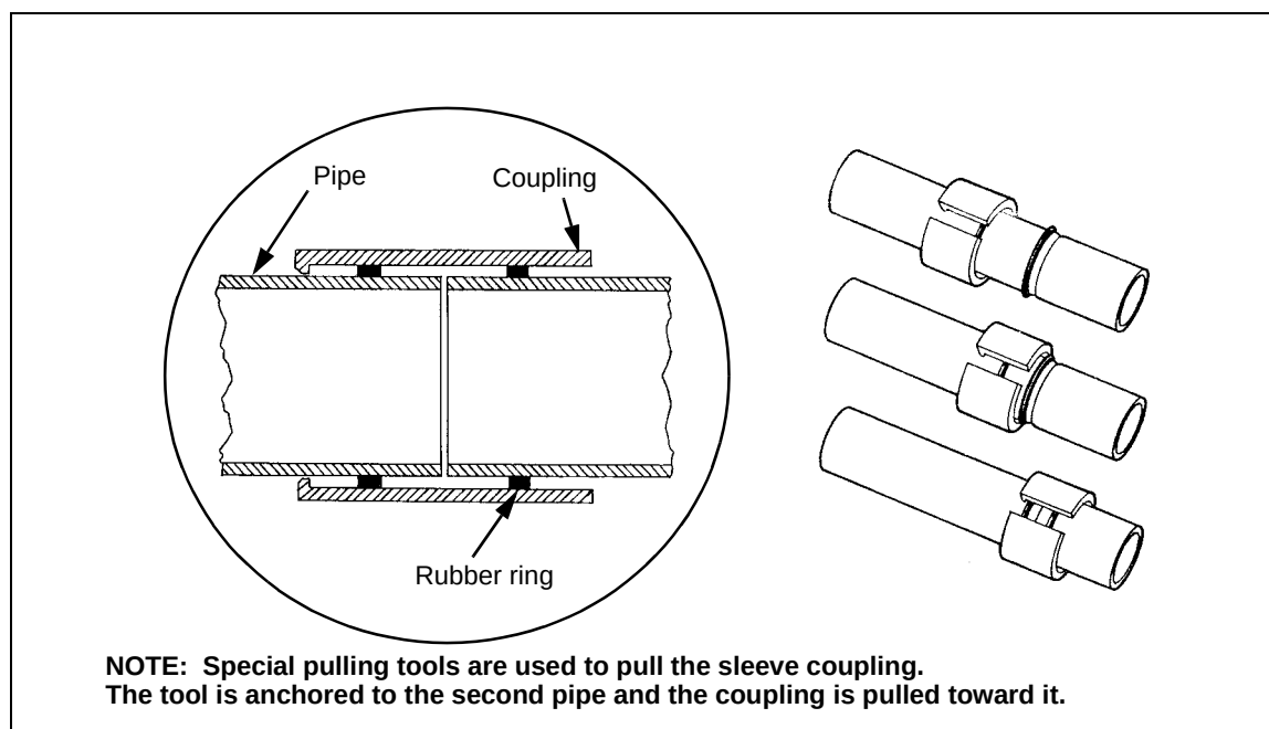
Figure 6-51. Cement-Pipe Coupling
