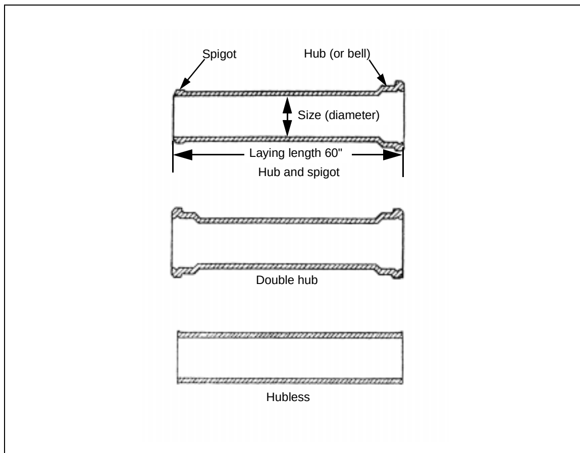
Figure 6-6. Cast-Iron Pipes
