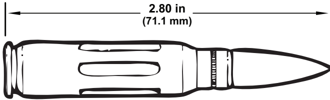
Figure 2-29. M63 Cartridge.
