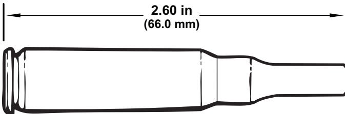
Figure 2-28. M82 Cartridge.
