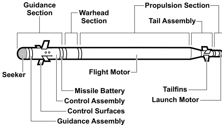
Figure 2-1. Stinger Missile.
