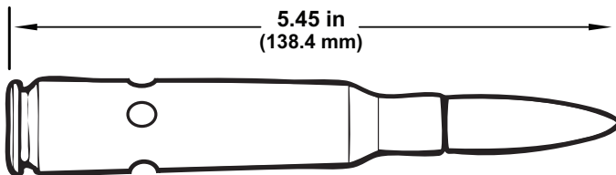
Figure 2-36. M2 Cartridge.
