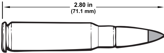
Figure 2-27. M62 Cartridge.
