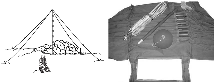
Figure 5-20. AS-2259/GR, Antenna.
