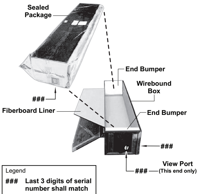
Figure 2-5. Missile Round Container.
