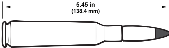
Figure 2-34. M17 Cartridge.
