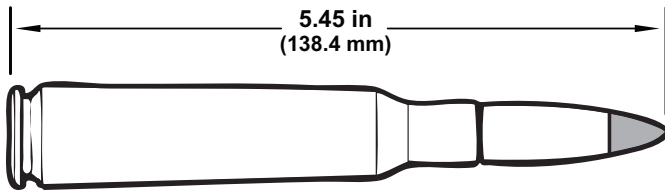
Figure 2-33. M1 Cartridge.
