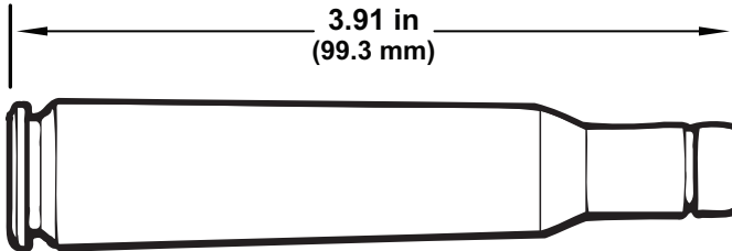
Figure 2-35. M1A1 Cartridge.
