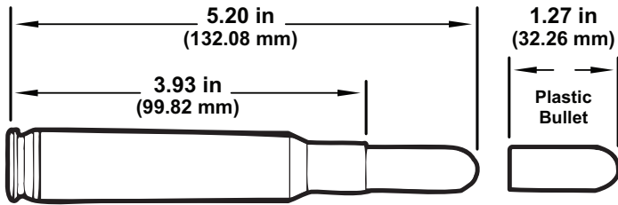
Figure 2-43. M858 Cartridge.
