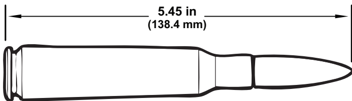
Figure 2-32. M2 or M33 Cartridge.
