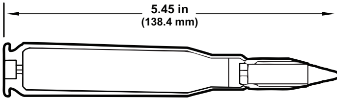
Figure 2-41. M903 Cartridge.
