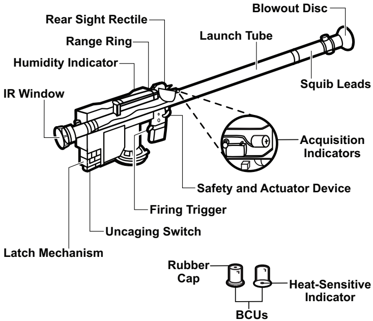
Figure 2-6. Stinger Weapon Round Components.
