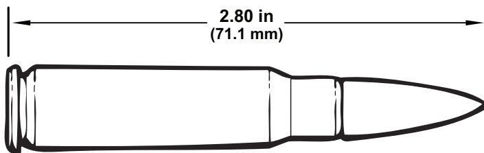
Figure 2-26. M80 Cartridge.
