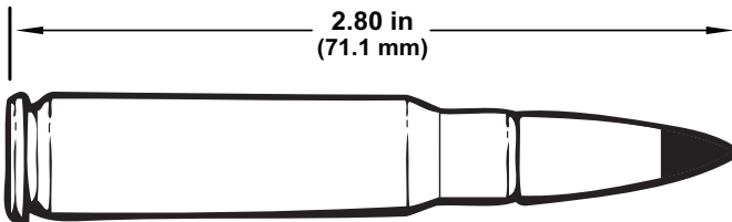
Figure 2-30. M61 Cartridge.
