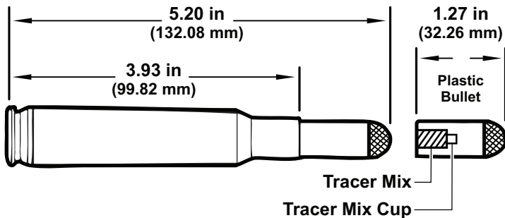
Figure 2-44. M860 Cartridge.
